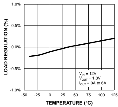
Load Regulation vs. Temperature
