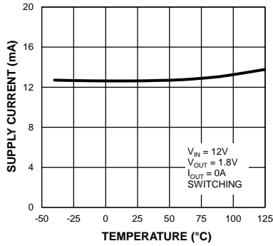
V IN Operating Supply Current vs. Temperature
