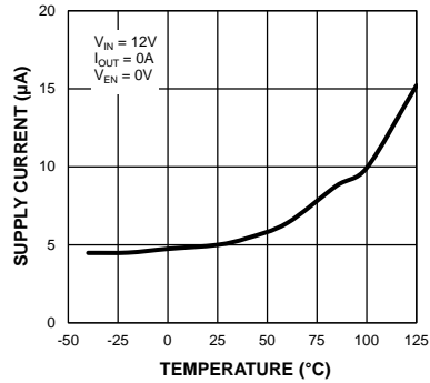
V IN Shutdown Current vs. Temperature
