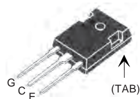
TO-3P (IXSQ)
