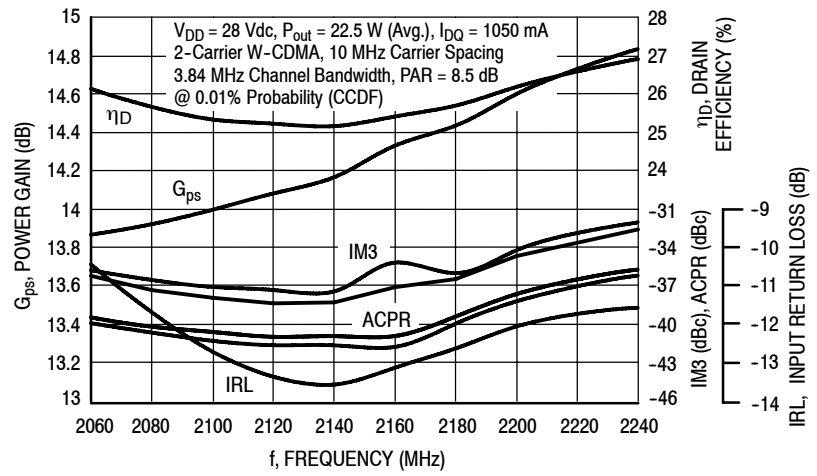
Figure 3. 2-Carrier W-CDMA Broadband Performance @ P out = 22.5 Watts Avg.
