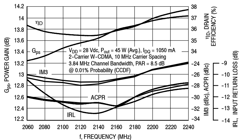
Figure 4. 2-Carrier W-CDMA Broadband Performance @ P out = 45 Watts Avg.
