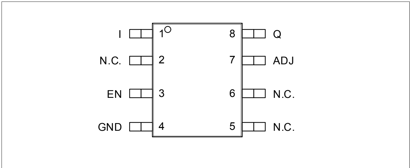
Figure 3 Pin Configuration TLS805B1 in PG-DSO-8 package
