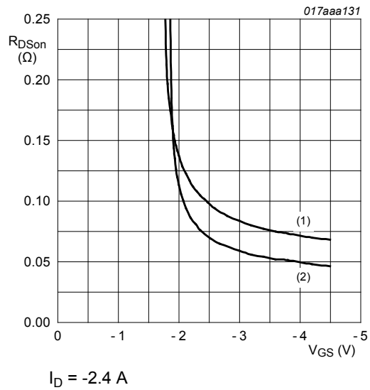
(1) T_j = 125\text{ }^\circ\text{C} (2) T_j = 25\text{ }^\circ\text{C} Fig. 9. Drain-source on-state resistance as a function of gate-source voltage; typical values
