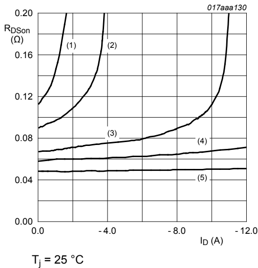
(1) V_{GS} = -1.8\text{ V} (2) V_{GS} = -2.0\text{ V} (3) V_{GS} = -2.25\text{ V} (4) V_{GS} = -3.0\text{ V} (5) V_{GS} = -4.5\text{ V} Fig. 8. Drain-source on-state resistance as a function of drain current; typical values
