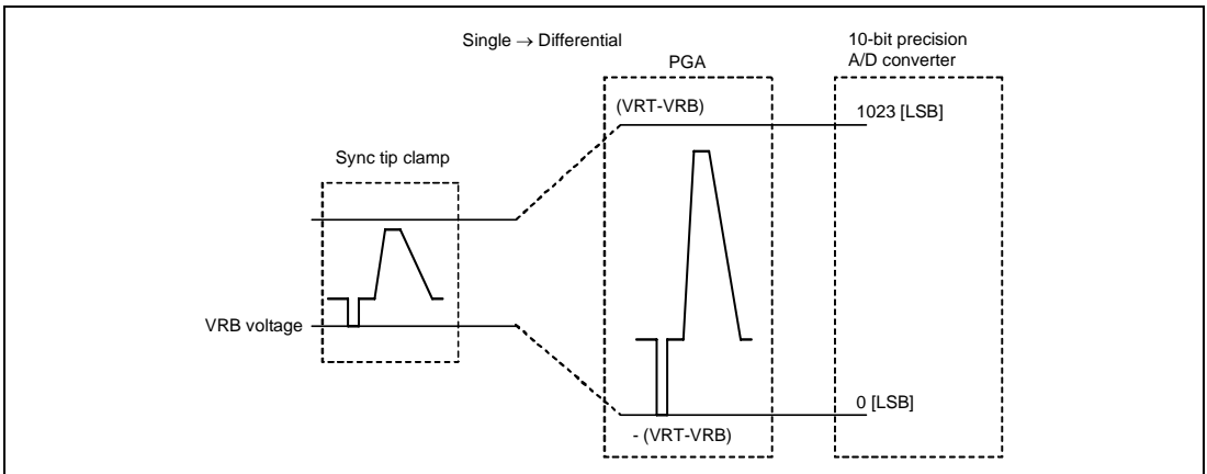
Figure 30.27 A/D Conversion Image
