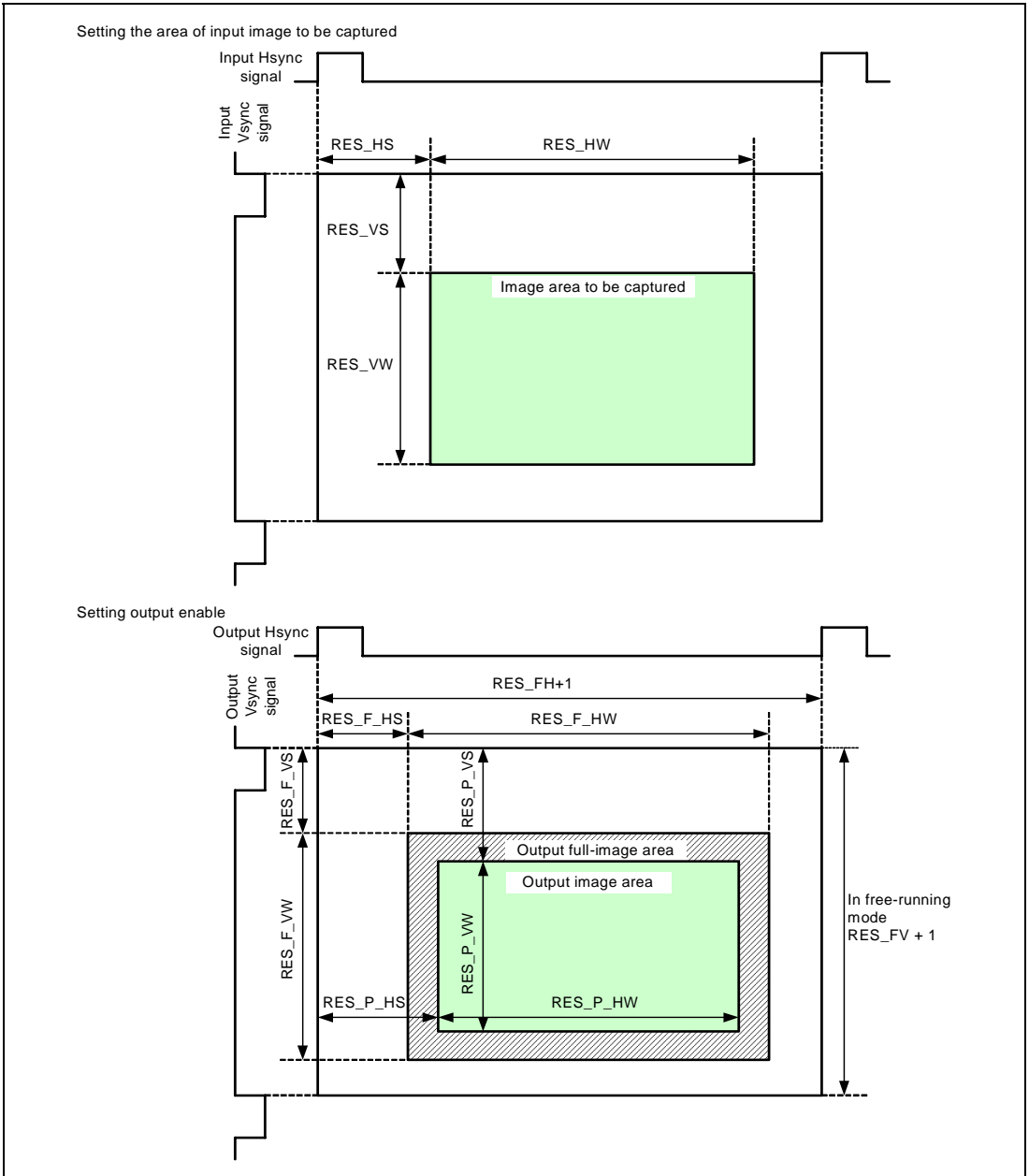
Figure 33.8 Enable Settings
