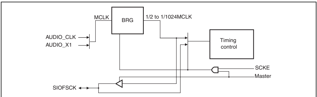
Figure 22.2 Serial Clock Supply
