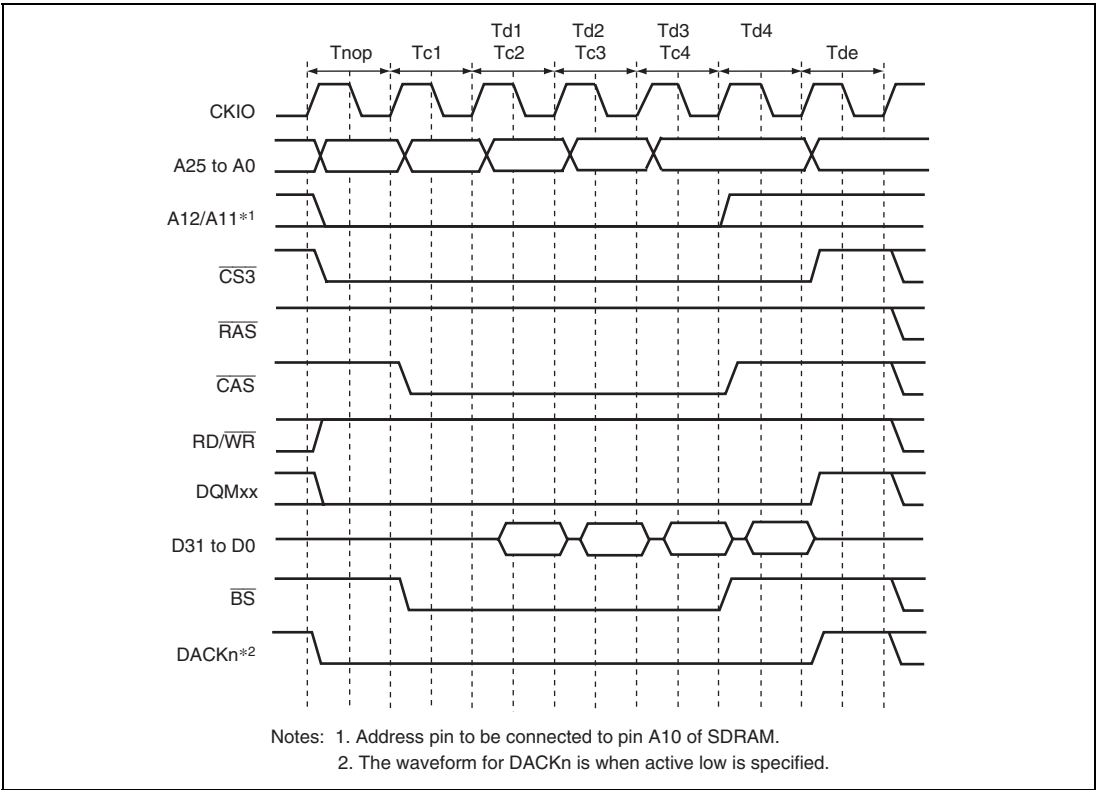
Figure 10.22 Burst Read Timing (Bank Active, Same Row Addresses in the Same Bank, CAS Latency 1)
