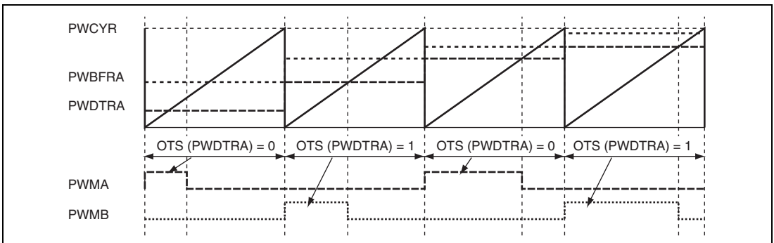
Figure 46.7 PWM Operation
