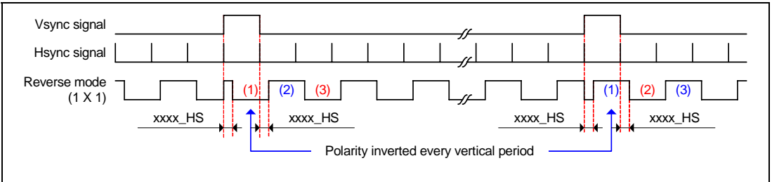
Figure 36.13 Horizontal Panel Driver Signal (in 1 × 1 Reverse Mode)
