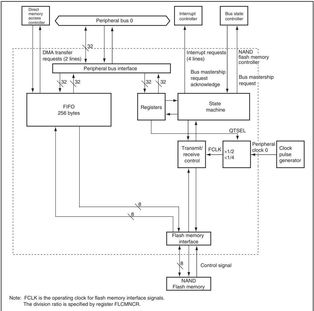
Figure 28.1 Block Diagram
