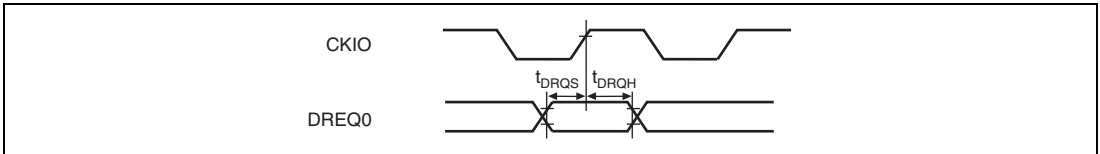
Figure 52.39 DREQ Input Timing
