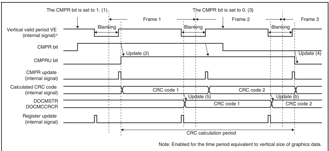
Figure 39.5 Register Update Timing
