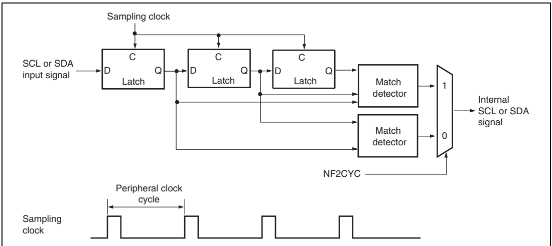
Figure 20.17 Block Diagram of Noise Filter
