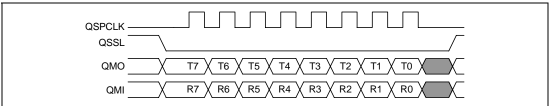
Figure 18.2 Transfer Format in Single-SPI Format
