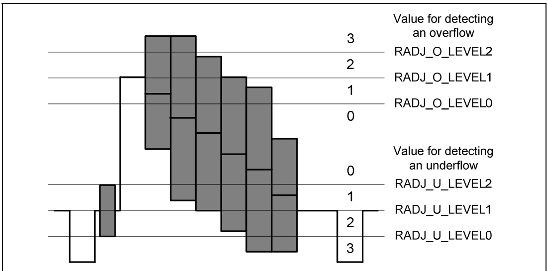
Figure 30.23 Over-Range Determination Areas
