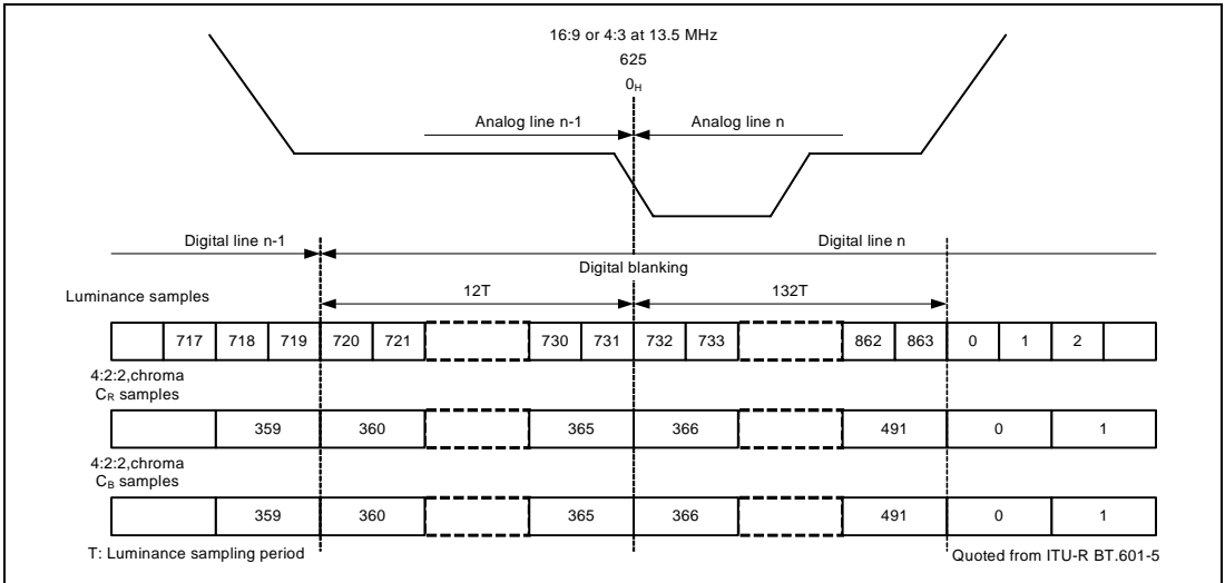
Figure 32.3 BT601 Horizontal Timing (625 Lines/50.00 Hz)
