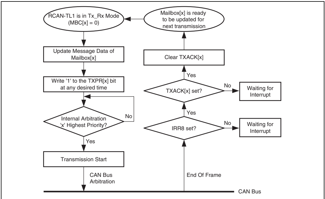
Figure 23.16 Transmission request
