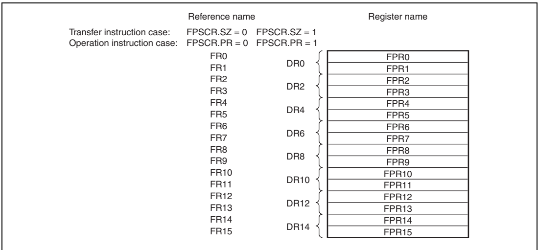
Figure 3.4 Floating-Point Registers
