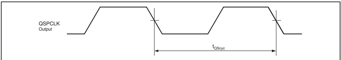
Figure 52.50 Clock Timing
