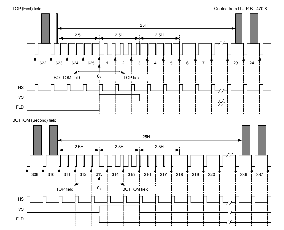
Figure 32.5 BT601 Vertical Timing (625 Lines/50.00 Hz)
