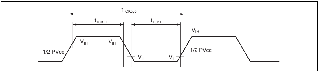
Figure 52.84 TCK Input Timing
