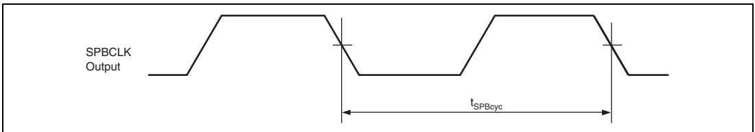
Figure 52.53 Clock Timing
