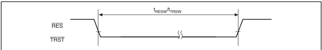
Figure 52.7 (1) Reset Input Timing
