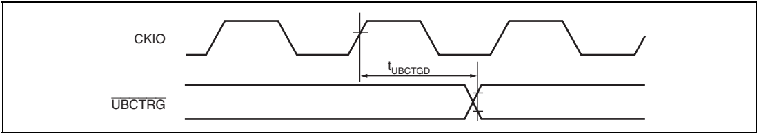
Figure 52.38 UBC Trigger Timing
