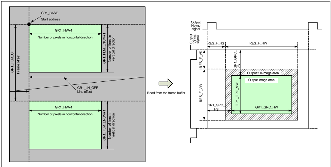
Figure 33.17 Area Setting for Graphics Display
