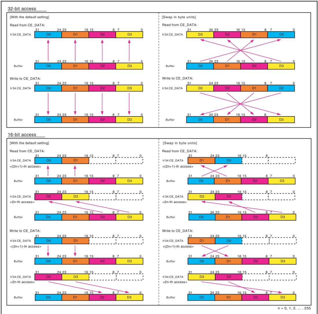
Figure 45.7 Specification of Byte-Swapping in 32/16-Bit Accesses (n = 1, 2, 3 ... 255)
