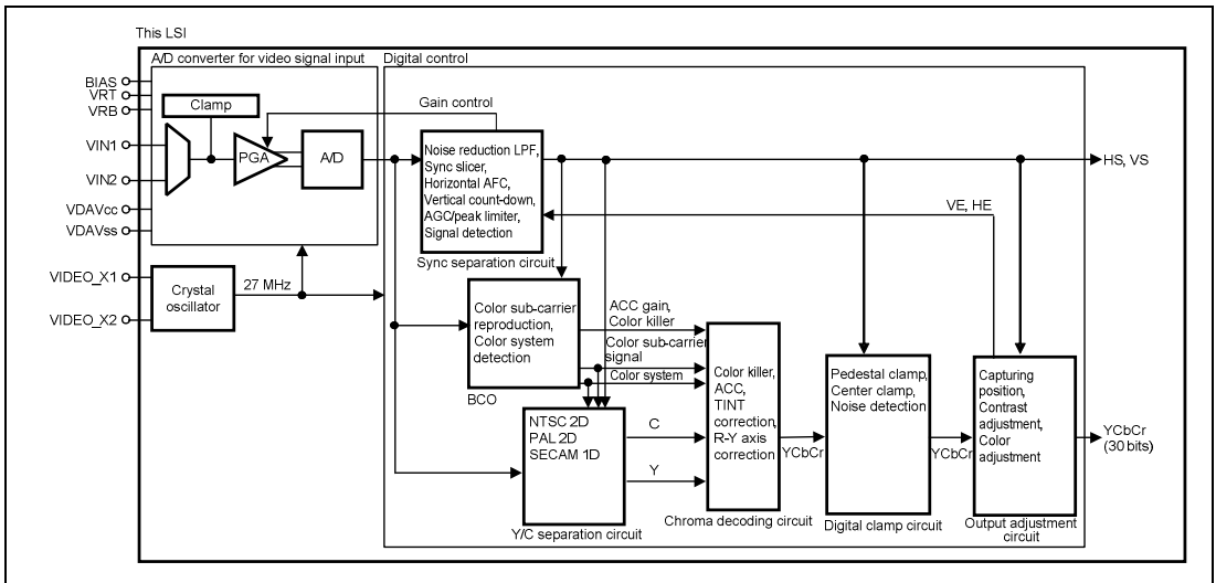
Figure 30.25 Overall Block Diagram
