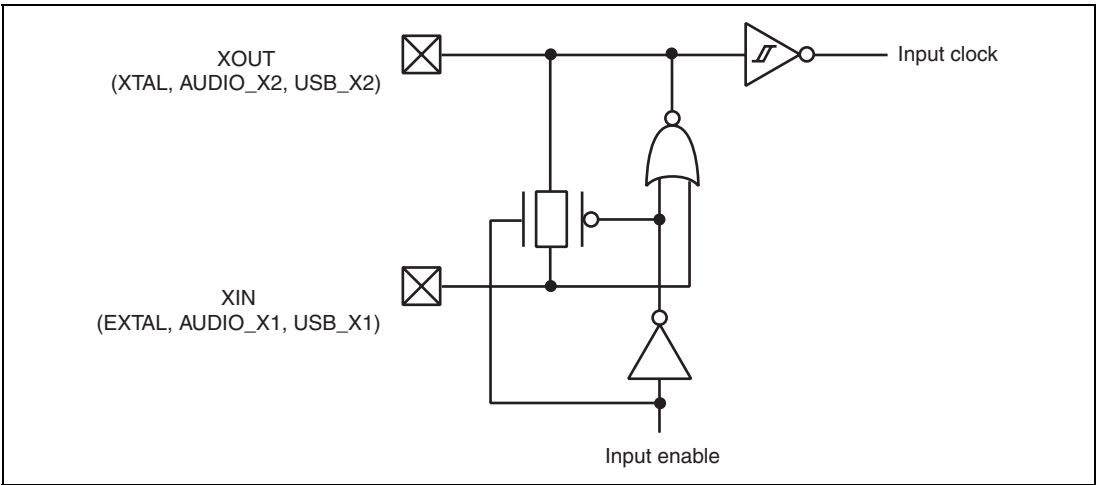
Figure 1.3 (10) Simplified Circuit Diagram (Oscillation Buffer 1)
