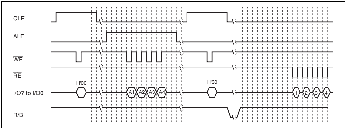
Figure 28.7 Read Operation Timing for NAND-Type Flash Memory
