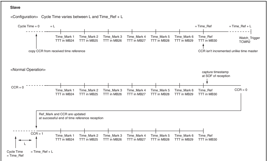
Figure 23.20 Time Slave
