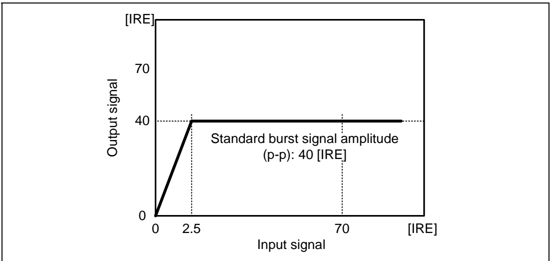
Figure 30.19 ACC Input/Output Characteristics
