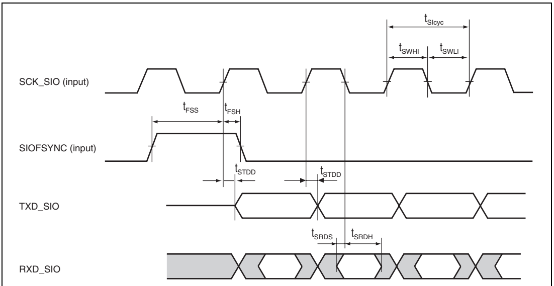
Figure 52.64 Transmission and Reception Timing (Slave Mode 1)
