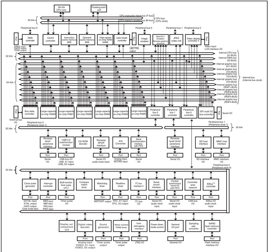
Figure 1.1 Block Diagram
