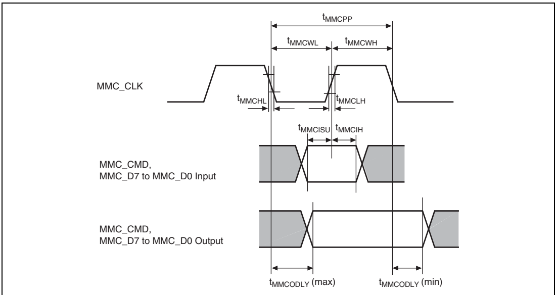
Figure 52.82 MMC Interface
