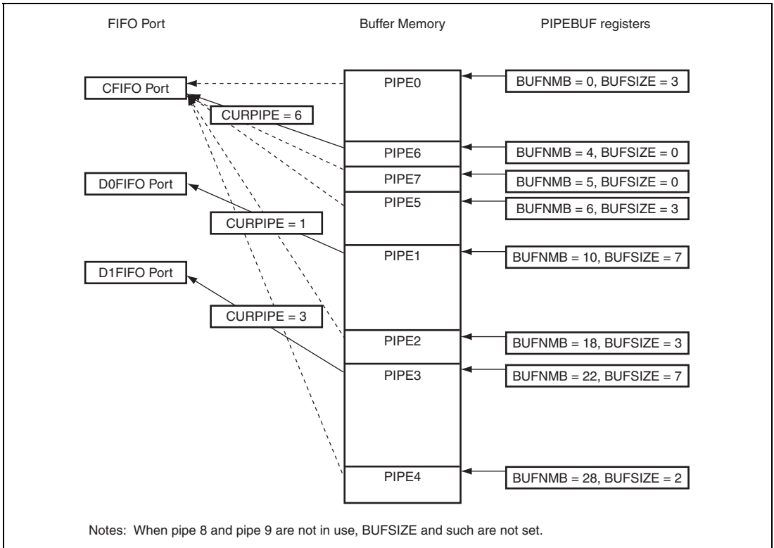
Figure 29.9 Example of a Buffer Memory Map
