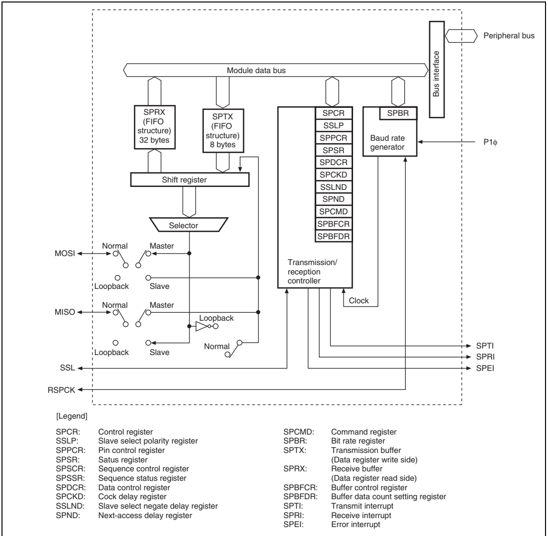
Figure 17.1 Block Diagram (for One Channel)
