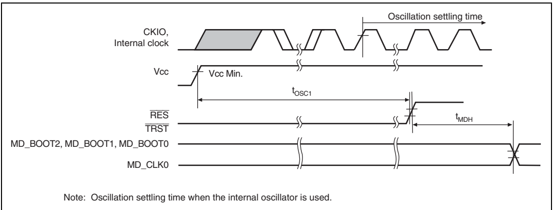
Figure 52.3 Power-On Oscillation Settling Time
