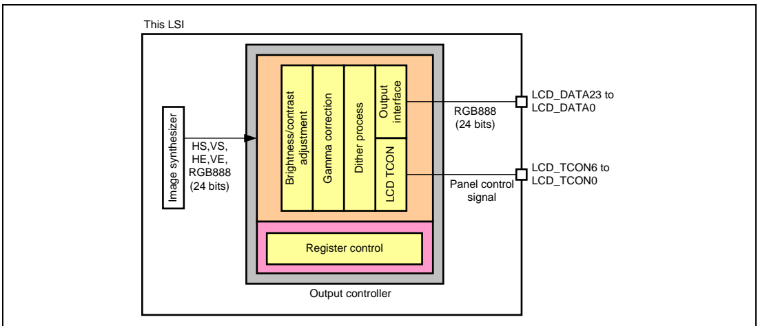
Figure 36.1 Functional Block Diagram of Output Controller
