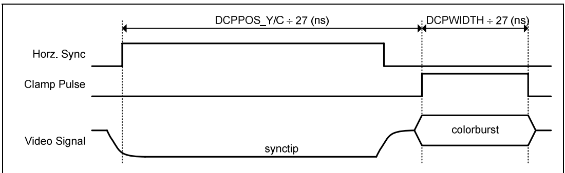
Figure 30.15 Digital Clamp Timing (Horizontal)
