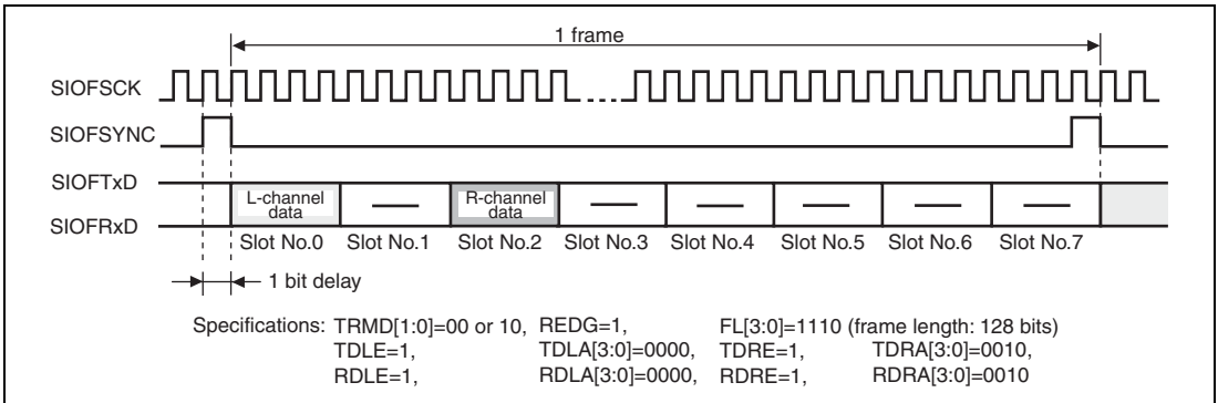
Figure 22.14 Transmit and Receive Timing (16-Bit Stereo Data (2))
