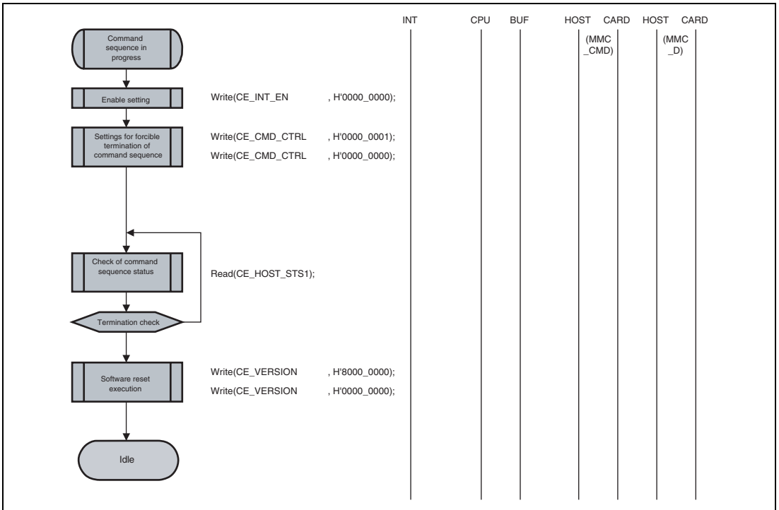
Figure 45.21 Forcible Termination
