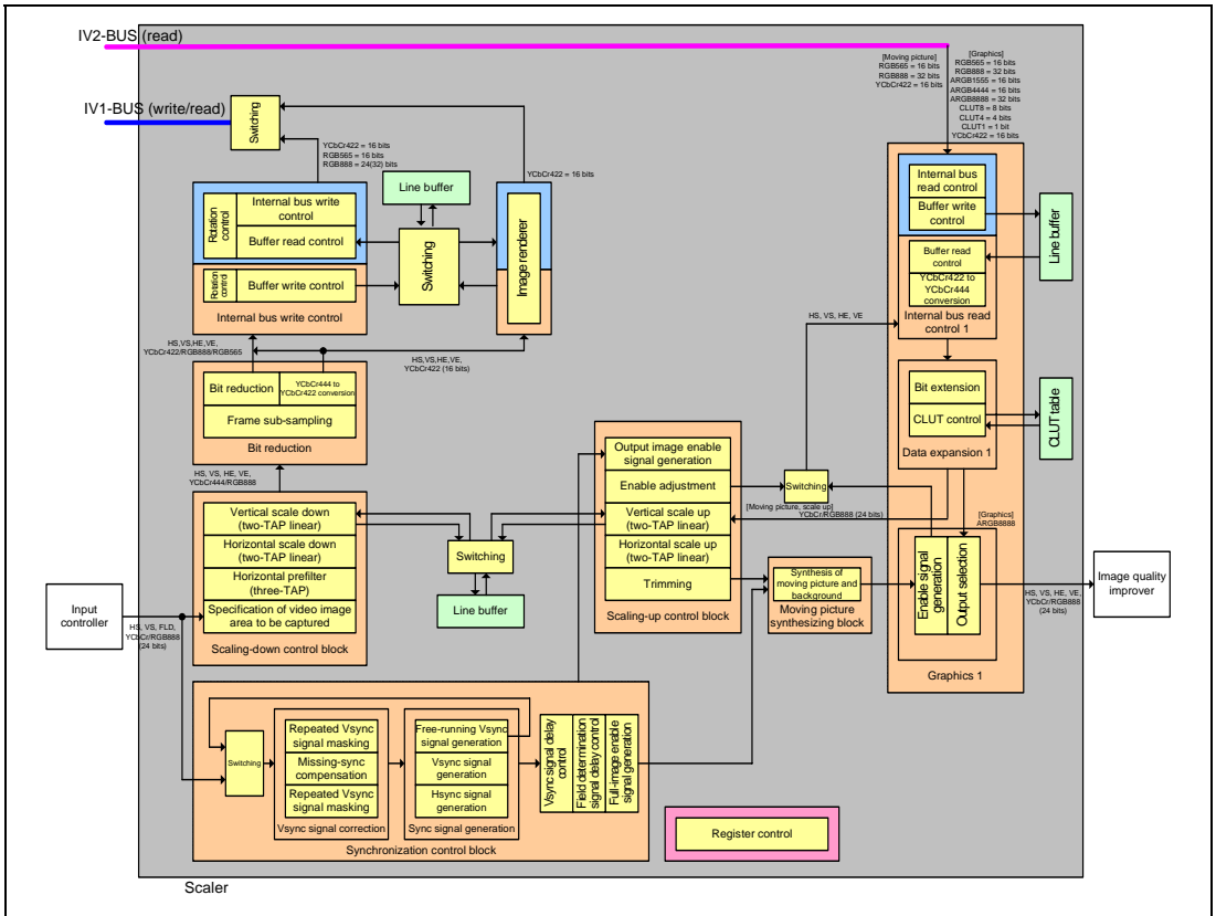
Figure 33.1 Functional Block Diagram of Scaler
