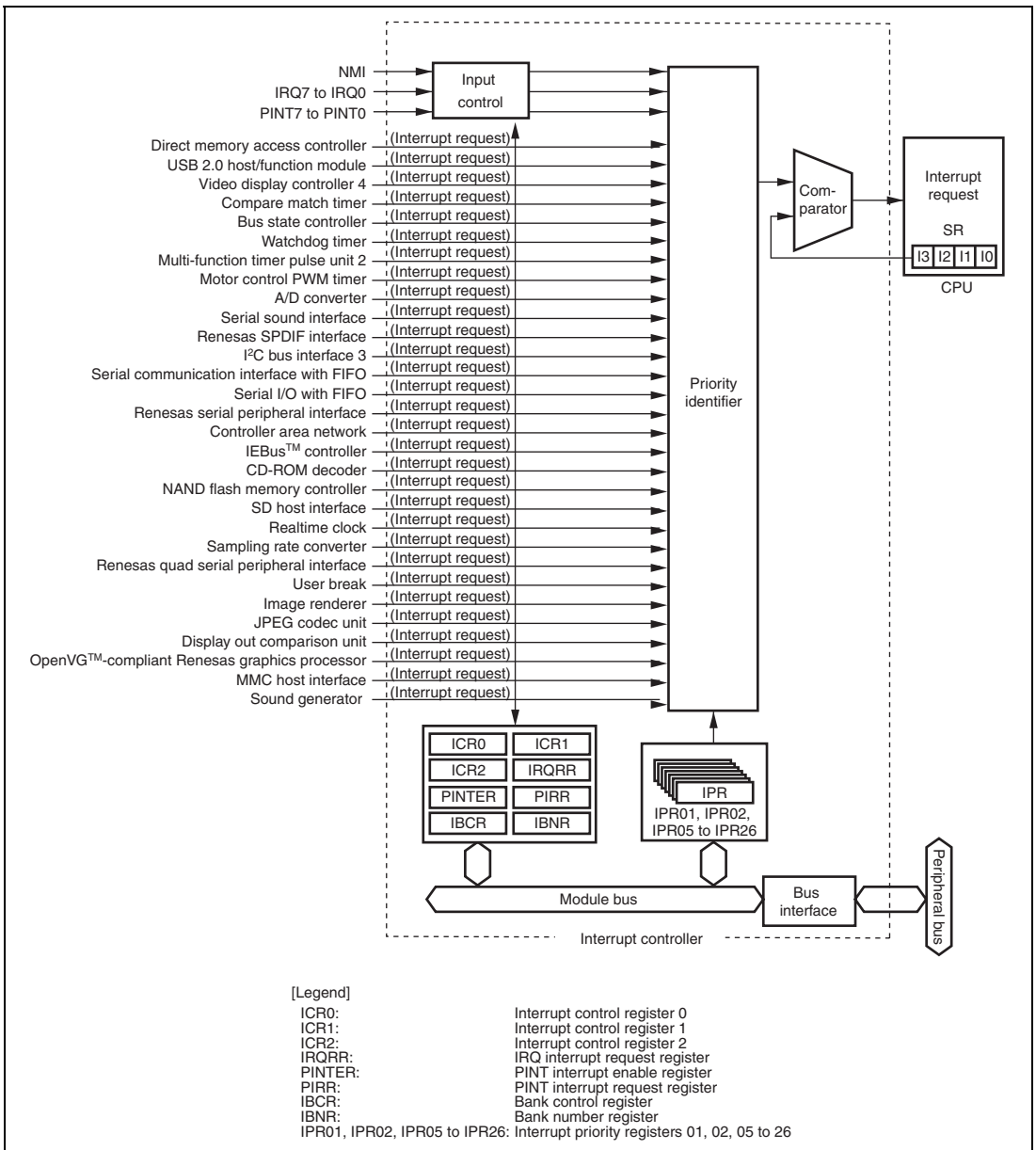
Figure 7.1 Block Diagram
