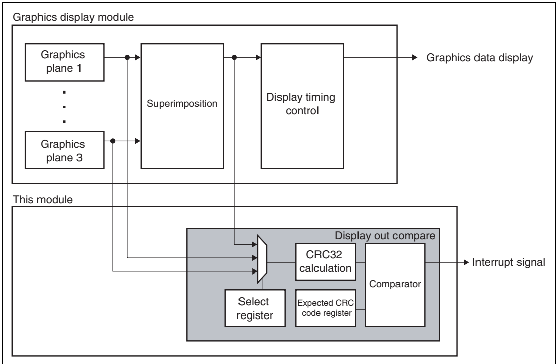
Figure 39.2 System Configuration
