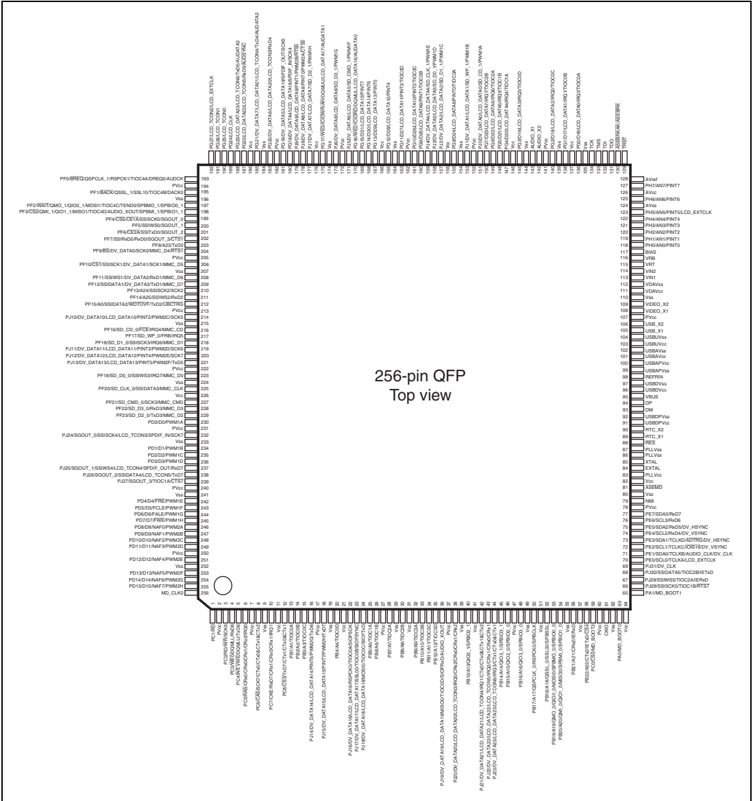
Figure 1.2 (2) Pin Assignment for the SH7269 Group (QFP)
