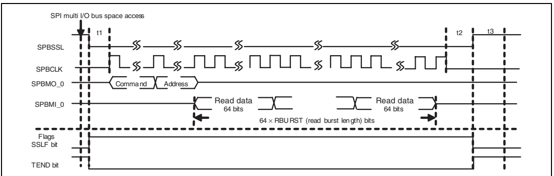
Figure 19.7 Burst Read Operation Timing (SSLE Bit = 0)
