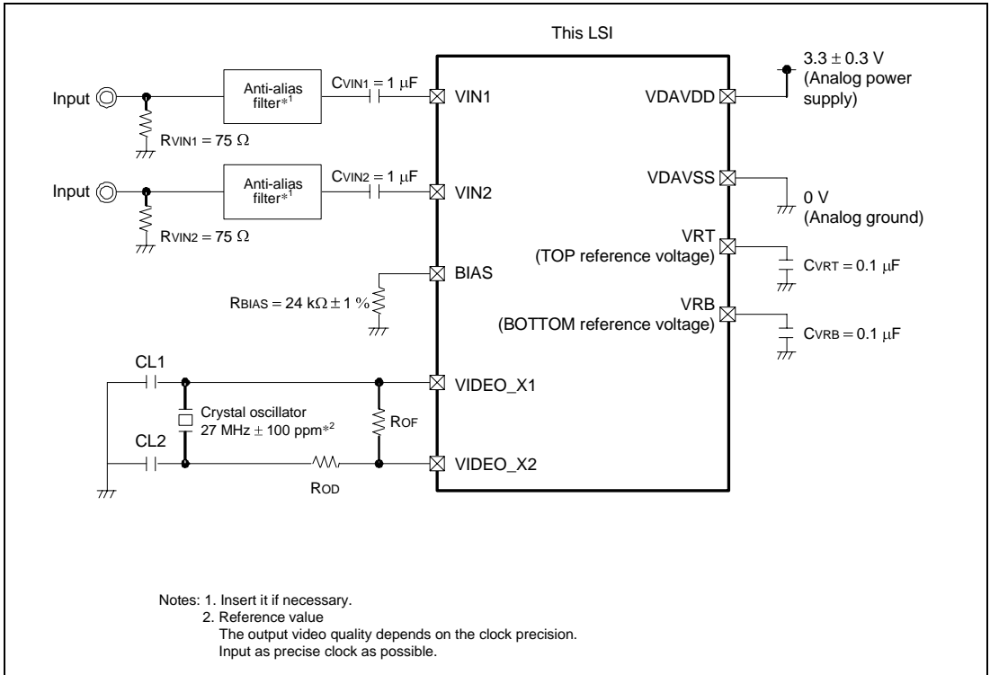
Figure 30.39 Pin Connection Example
