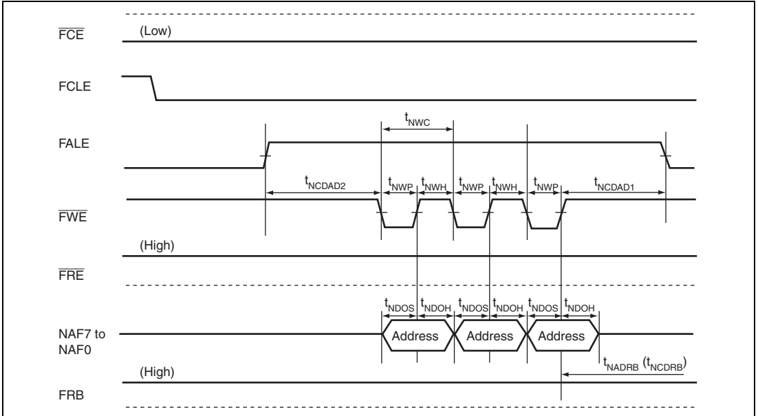
Figure 52.67 NAND Type Flash Memory Address Issuance Timing
