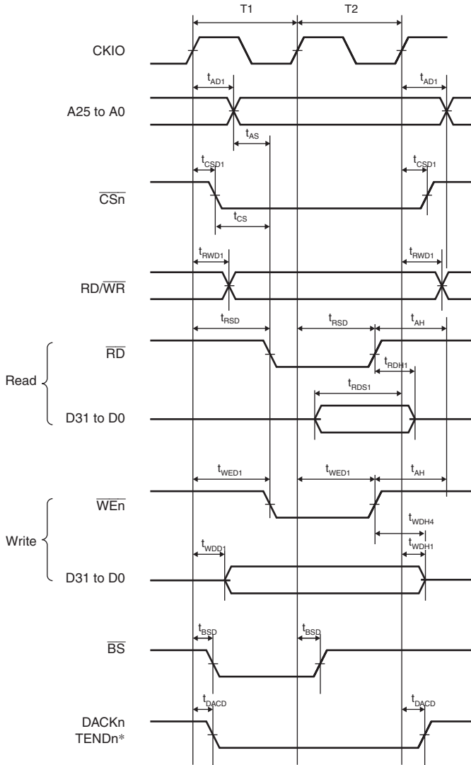
Figure 52.9 Basic Bus Timing for Normal Space (No Wait)
