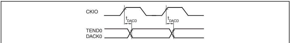
Figure 52.40 DACK, TEND Output Timing
