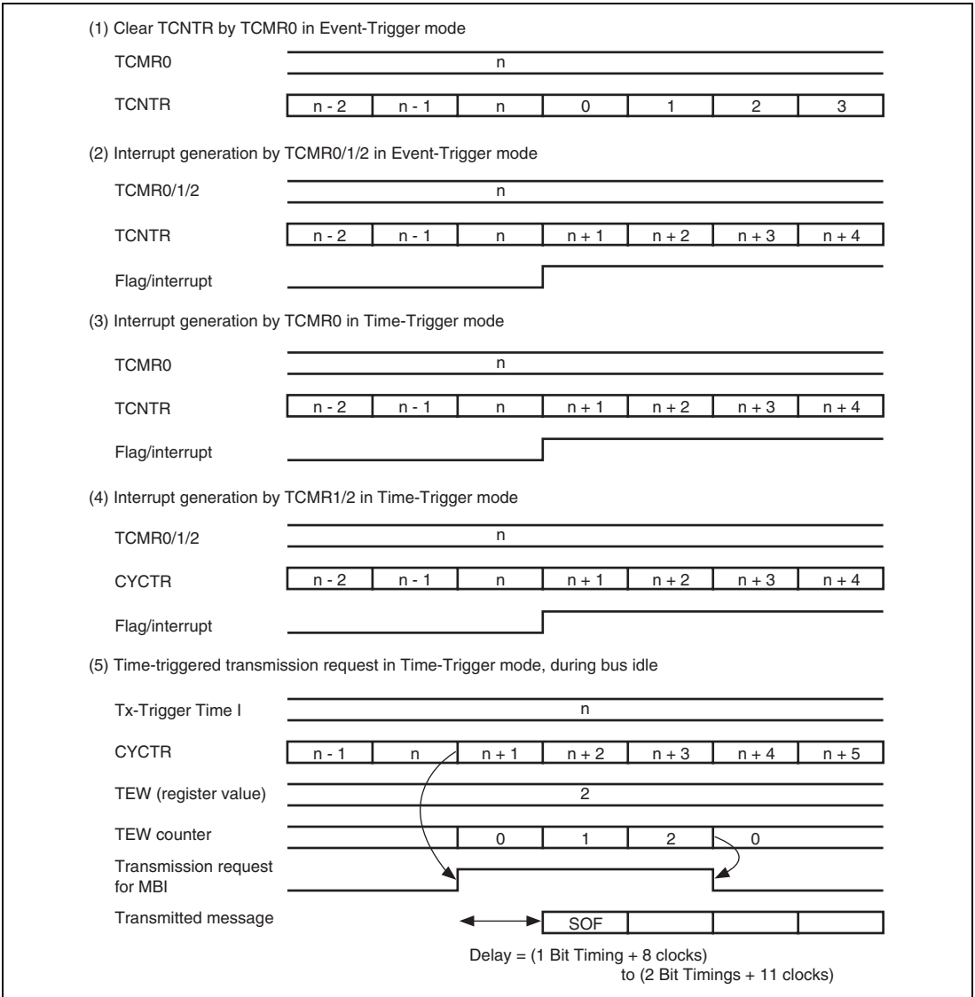
Figure 23.23 Timing Diagram of Timer
