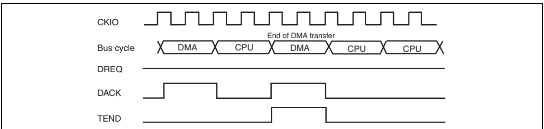
Figure 11.15 Example of DMA Transfer End Signal Timing (Cycle Steal Mode Level Detection)
