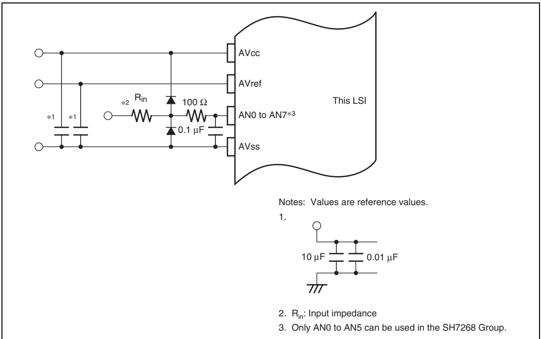
Figure 27.8 Example of Analog Input Protection Circuit
