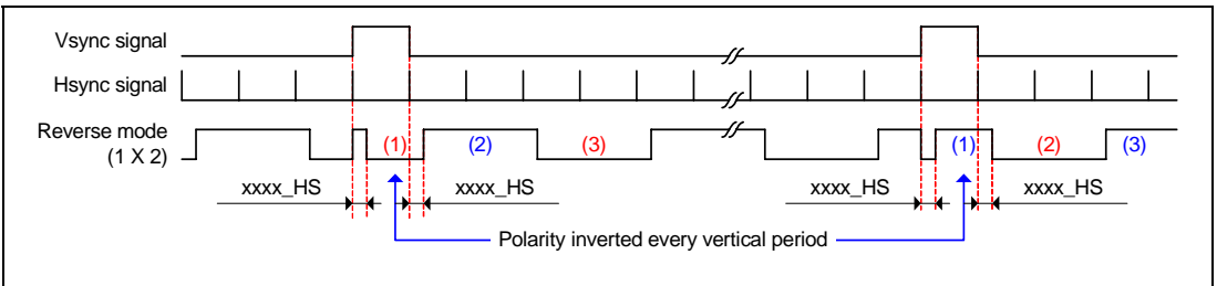
Figure 36.14 Horizontal Panel Driver Signal (in 1 × 2 Reverse Mode)
