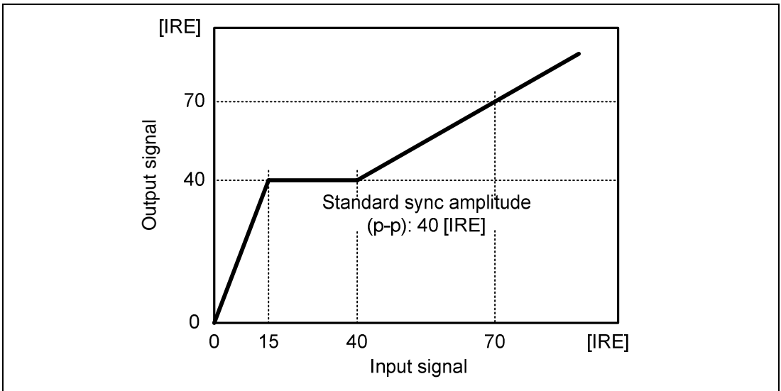
Figure 30.22 AGC Characteristics (Sync Signal Amplitude Reference)
