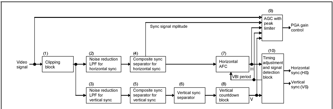
Figure 30.28 Block Diagram of Sync Separator Circuit
