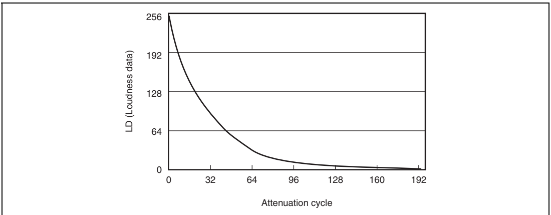
Figure 43.4 Attenuation Characteristics
