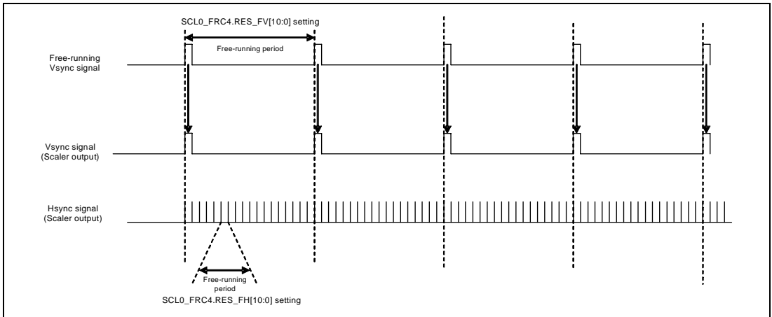
Figure 31.4 Free Running Vsync Timing
