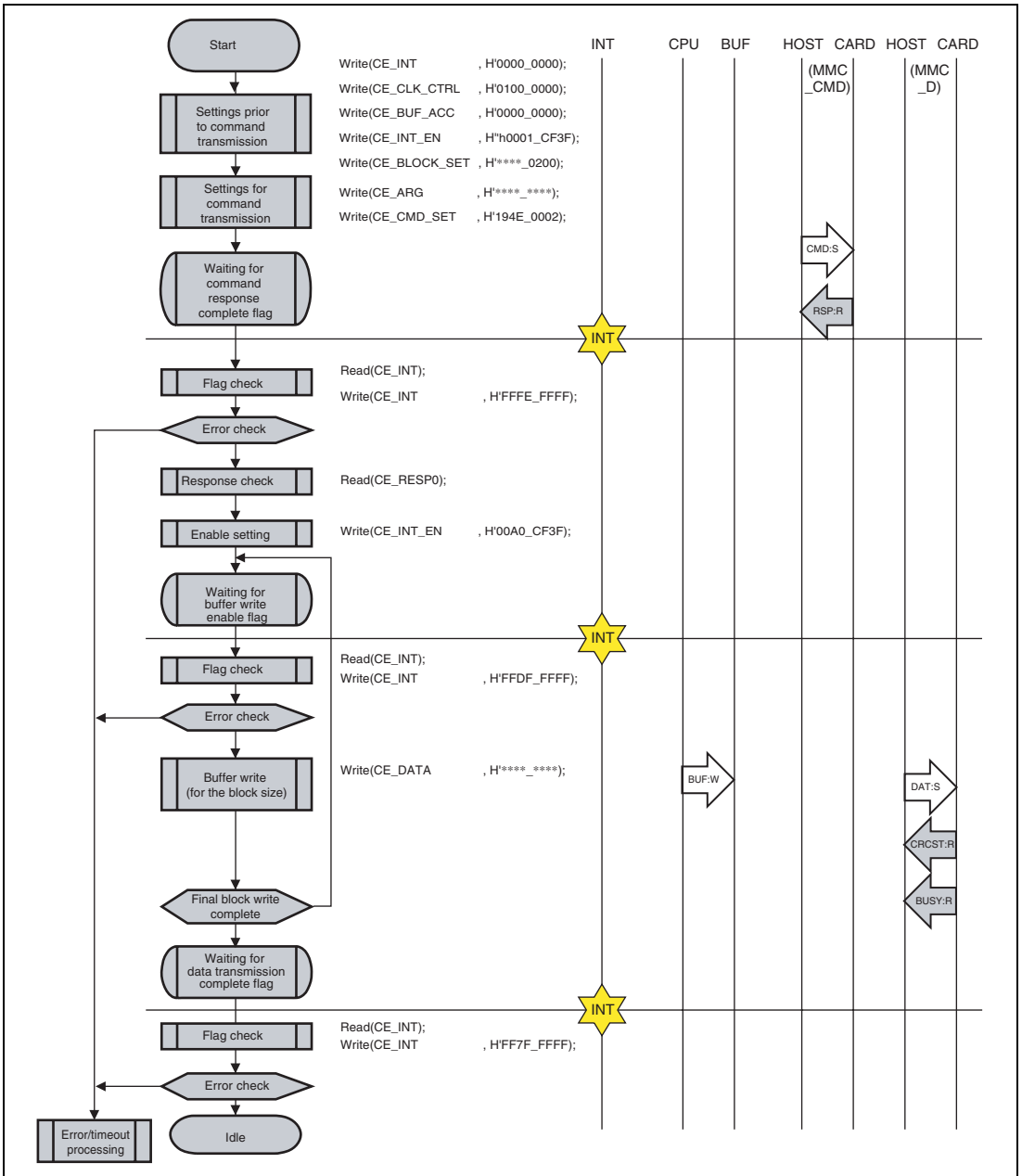
Figure 45.19 Multi-Block Write (CMD25 Pre-Defined)
