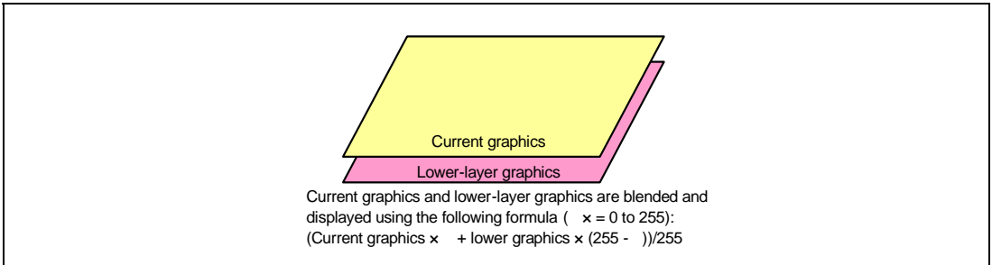
Figure 35.9 Graphics Planes with GR_DISP_SEL Set to 3
