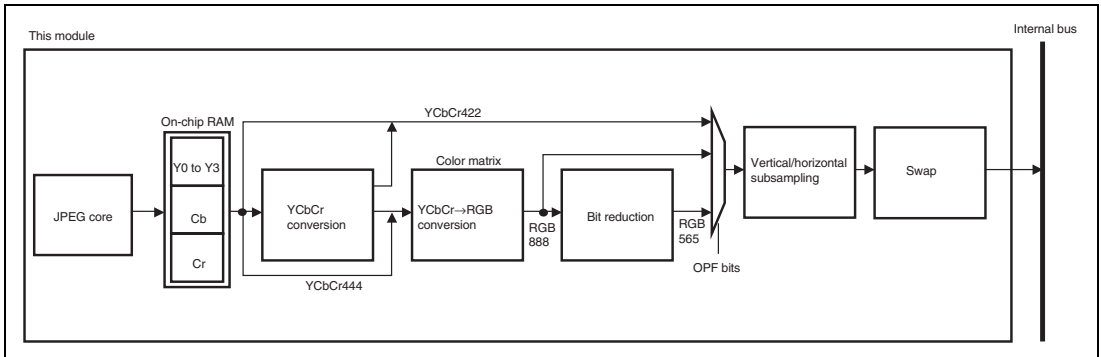
Figure 41.12 Block Diagram of Output Pixel Format Conversion in Decompression
