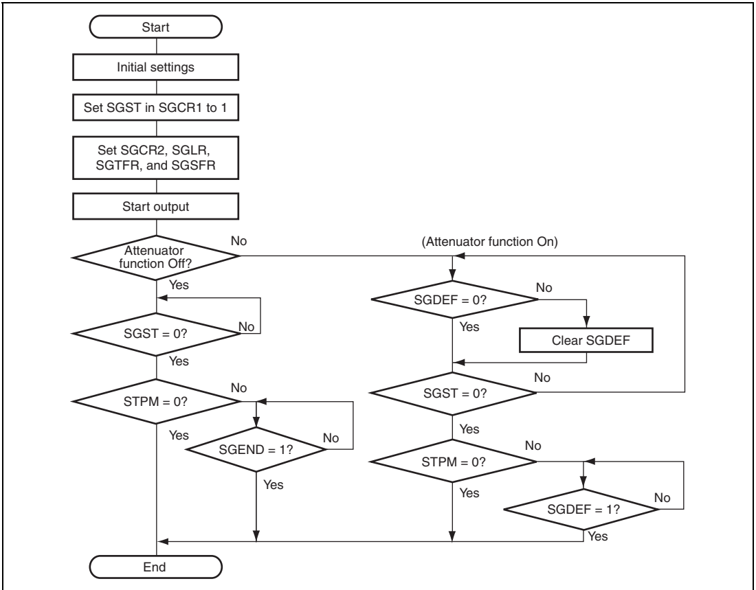
Figure 43.3 Operation Flow
