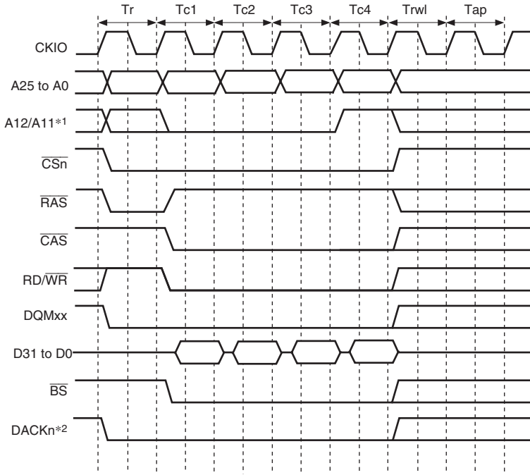
Figure 10.19 Basic Timing for Burst Write (Auto Pre-Charge)
