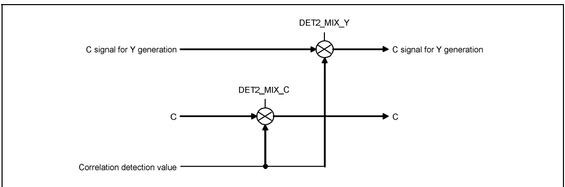
Figure 30.34 Configuration of Correlation Detection Value Mixing Block
