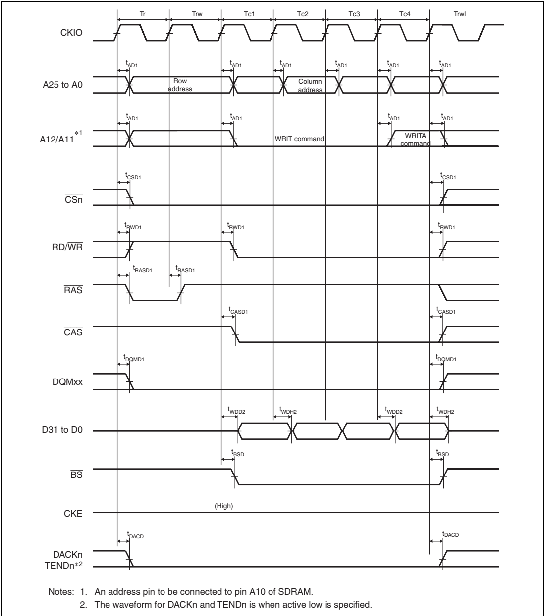
Figure 52.24 Synchronous DRAM Burst Write Bus Cycle (Four Write Cycles) (Auto Precharge, WTRCD = 1 Cycle, TRWL = 1 Cycle)
