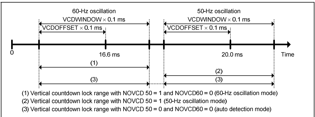
Figure 30.13 Vertical Countdown Lock Ranges
