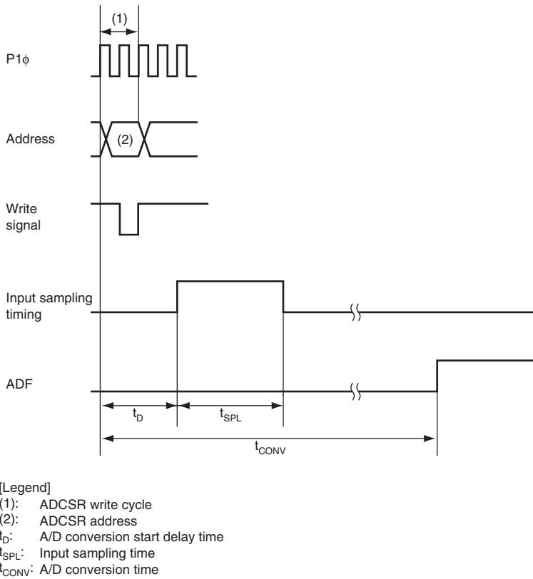
Figure 27.5 A/D Conversion Timing
