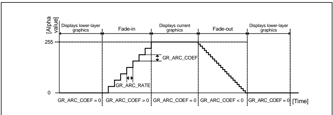
Figure 35.11 Fade In and Fade Out
