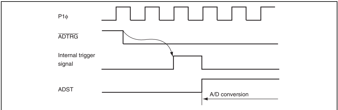
Figure 27.6 External Trigger Input Timing
