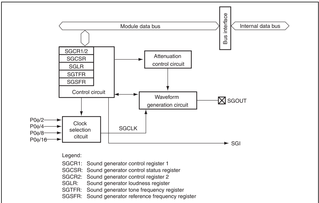
Figure 43.1 Block Diagram
