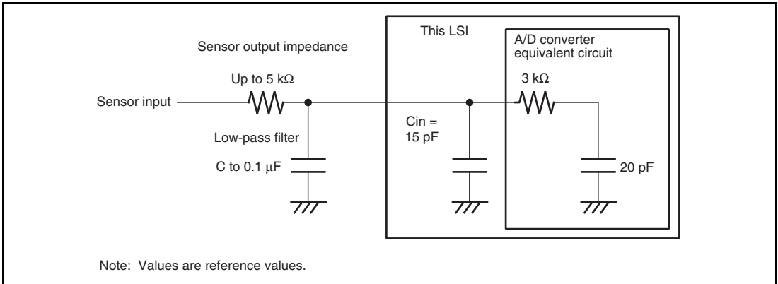
Figure 27.10 Example of Analog Input Circuit
