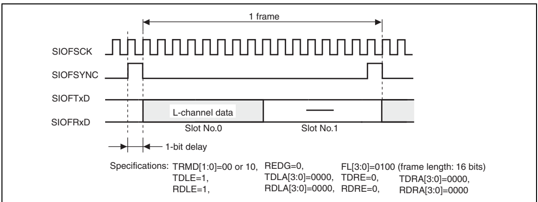
Figure 22.11 Transmit and Receive Timing (8-Bit Monaural Data (2))
