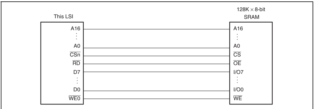
Figure 10.7 Example of 8-Bit Data-Width SRAM Connection
