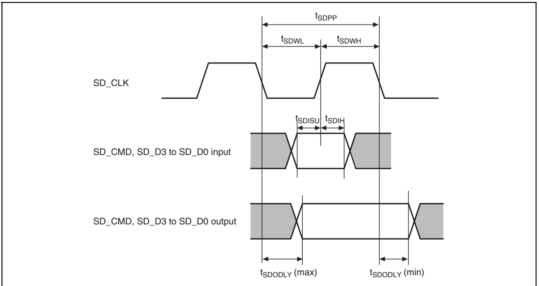
Figure 52.81 SD Card Interface
