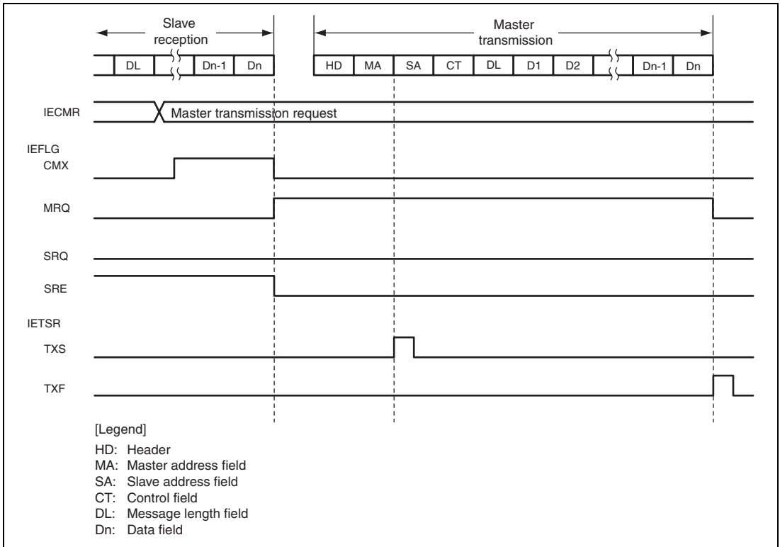
Figure 24.13 Master Transmit Operation Timing
