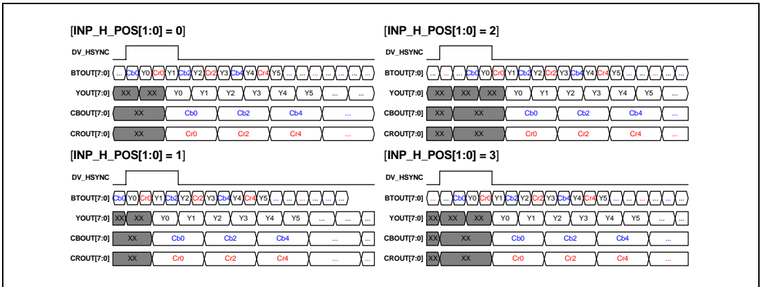
Figure 32.11 YCbCr Data Expansion for BT656/BT601 Input
