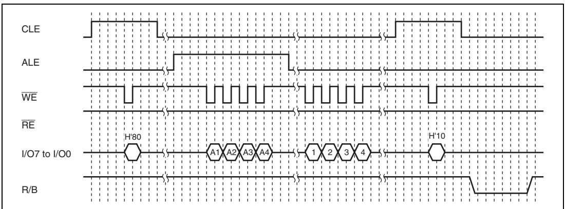
Figure 28.8 Programming Operation Timing for NAND-Type Flash Memory (1)
