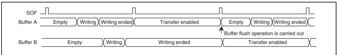
Figure 29.21 Example of Buffer Flush Function Operation
