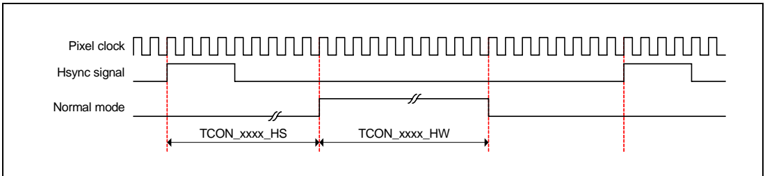
Figure 36.10 Horizontal Panel Driver Signal (in Normal Mode)
