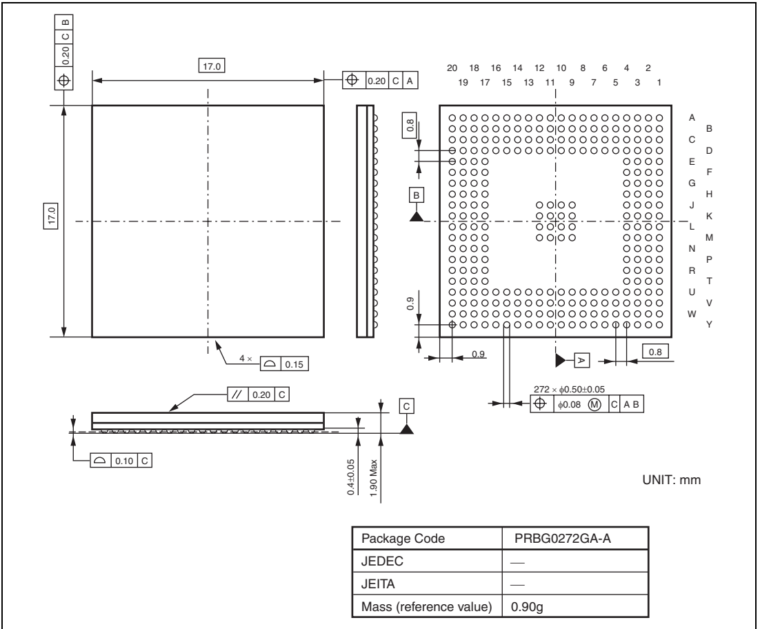
Figure A.3 SH7269 (BGA Version)
