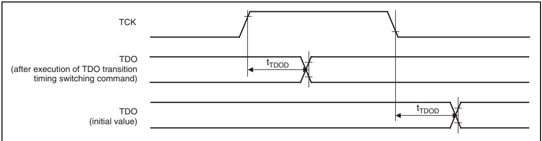
Figure 50.3 User Debugging Interface Data Transfer Timing
