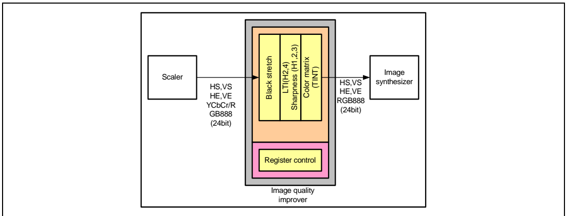
Figure 34.1 Functional Block Diagram of Image Quality Improver
