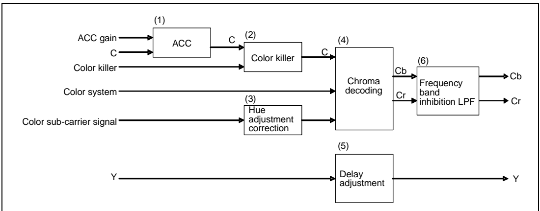
Figure 30.36 Block Diagram of Chroma Decoding Circuit
