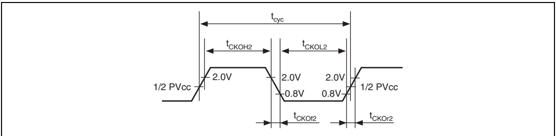
Figure 52.2 (2) CKIO Clock Output Timing 2
