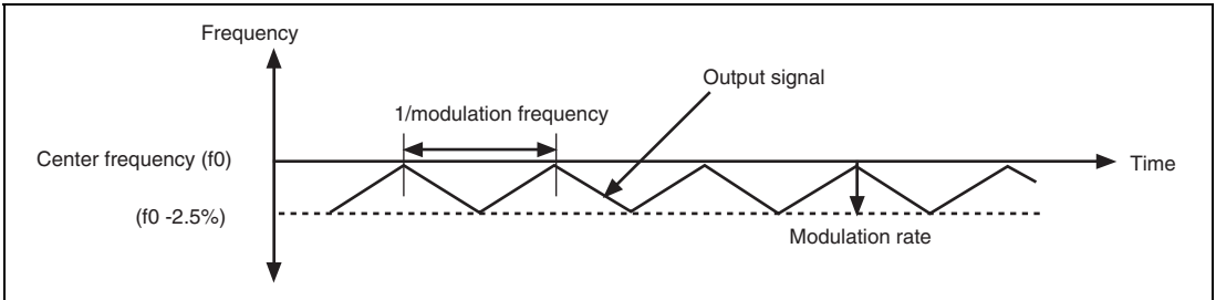
Figure 5.4 Definition of SSCG Modulation Rate and Frequency
