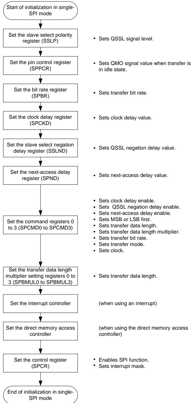
Figure 18.14 Example of Initialization Flowchart in Single-SPI Mode
