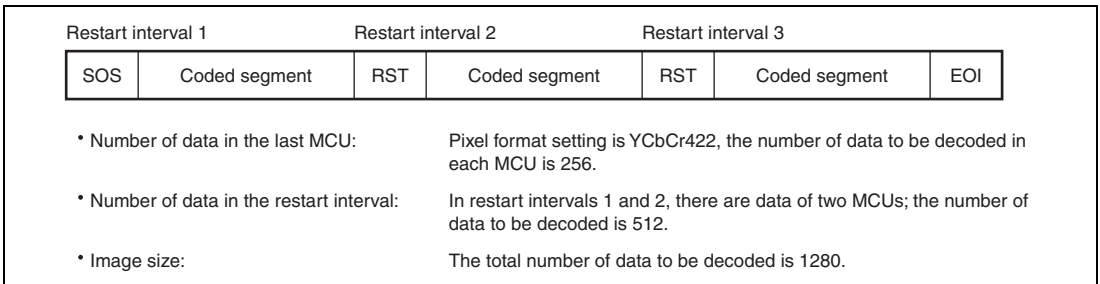
Figure 41.11 Huffman Coded Segment
