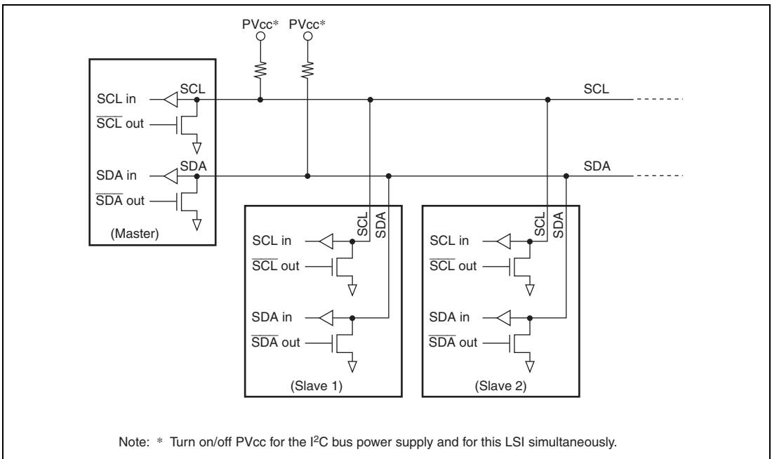
Figure 20.2 External Circuit Connections of I/O Pins
