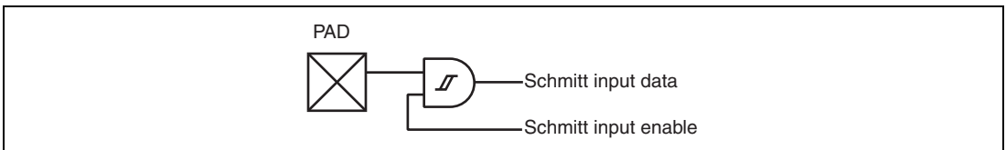
Figure 1.3 (3) Simplified Circuit Diagram (Schmitt AND Input Buffer)
