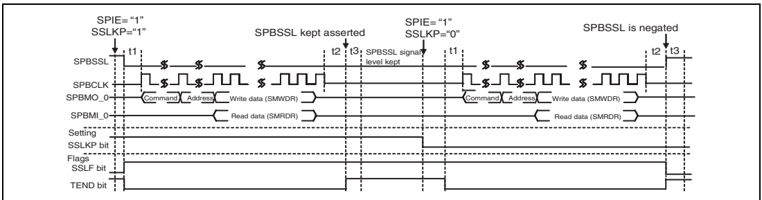
Figure 19.13 Data Transfer Timing using the SSLKP Bit
