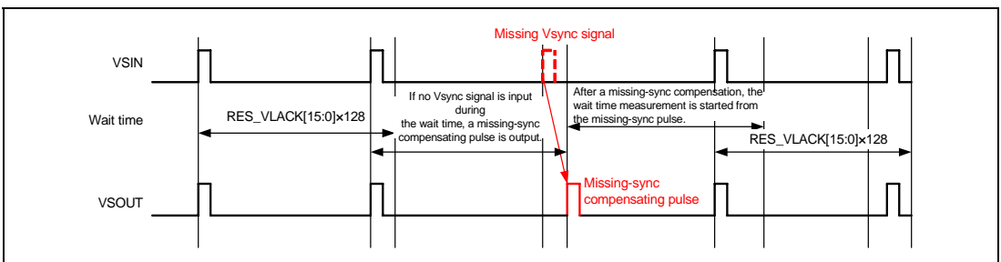
Figure 33.3 Compensation of Missing Vsync Signals
