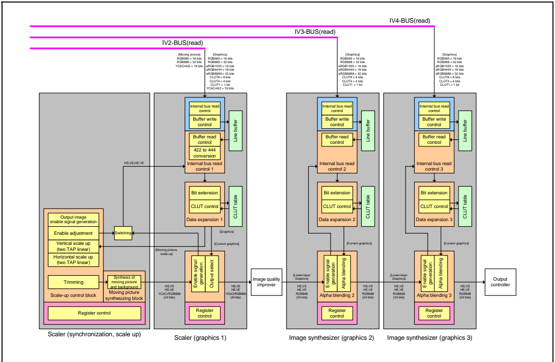
Figure 35.1 Functional Block Diagram of Image Synthesizer
