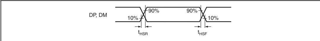
Figure 52.75 DP and DM Output Timing (High-Speed)
