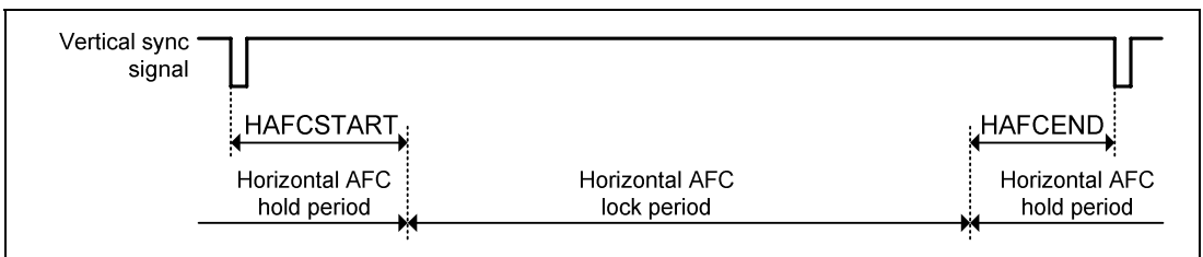
Figure 30.12 Horizontal AFC Lock Range (Vertical)
