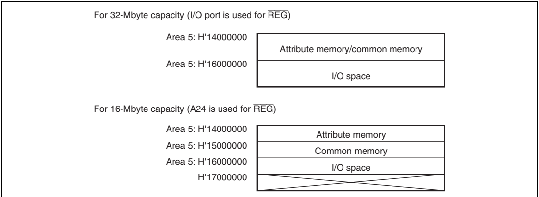
Figure 10.42 Example of PCMCIA Space Allocation (CS5WCR.SA[1:0] = B'10)
