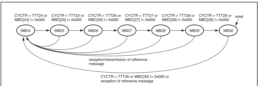
Figure 23.13 TTTSEL modification algorithm
