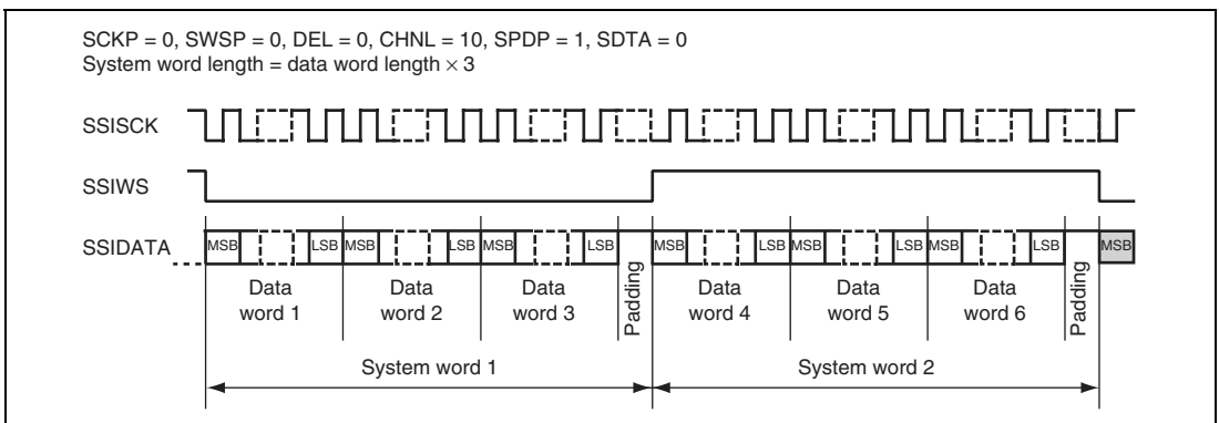
Figure 21.7 Multi-Channel Format (6 Channels with High Padding)
