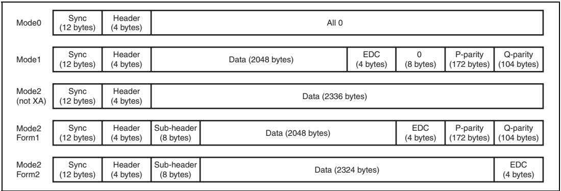
Figure 26.1 Formats Supported by CD-ROM Decoder
