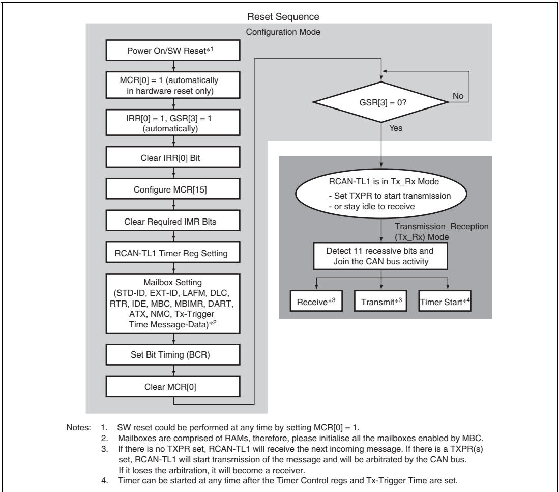
Figure 23.14 Reset Sequence
