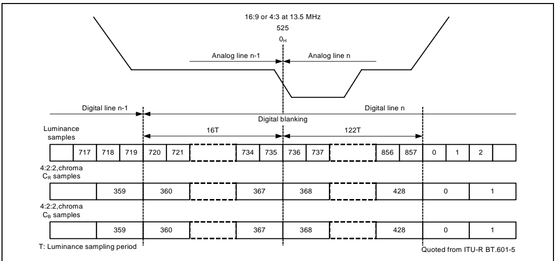
Figure 32.4 BT601 Horizontal Timing (525 Lines/59.94 Hz)
