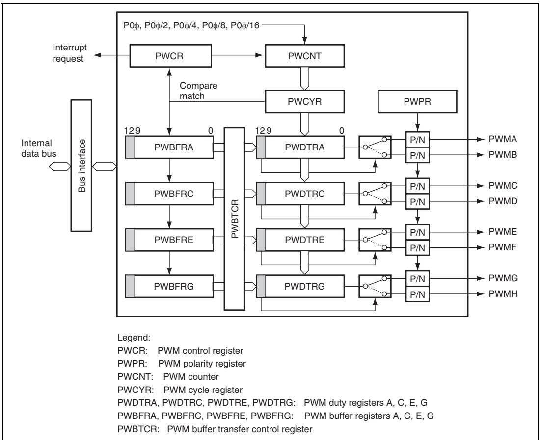
Figure 46.1 Block Diagram of Motor Control PWM Timer
