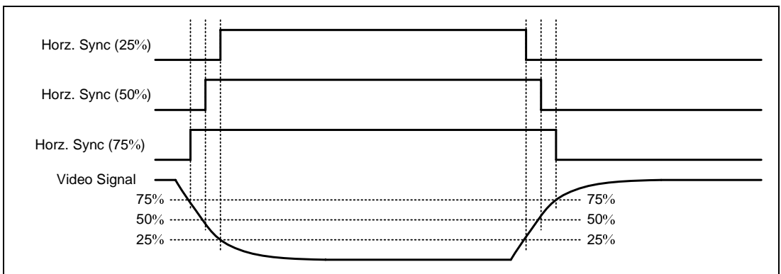
Figure 30.9 Auto Slice Level Setting
