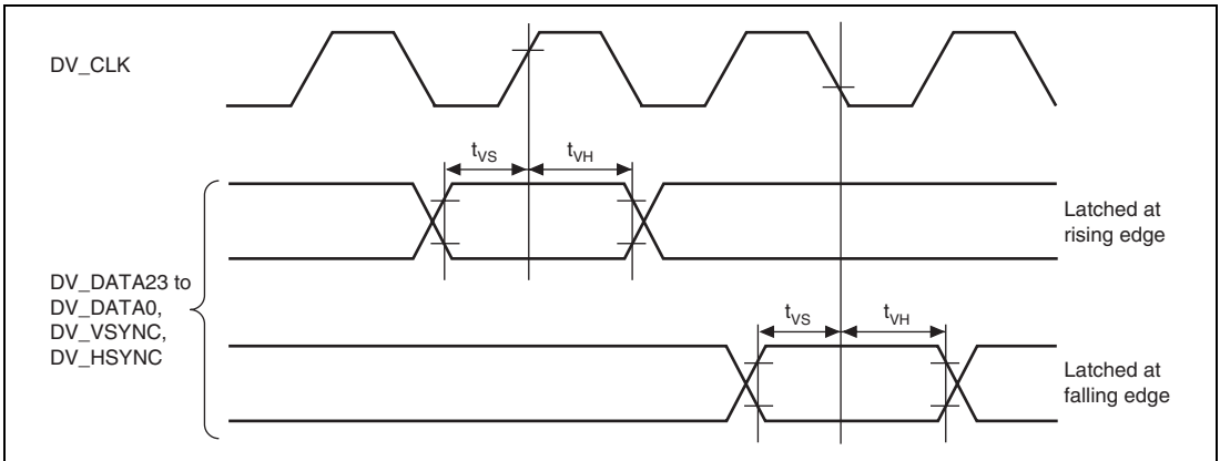
Figure 52.79 Video Input Timing
