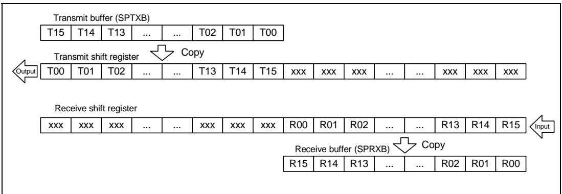
Figure 18.9 LSB First Transfer (16-Bit Data)
