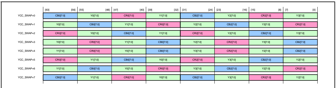
Figure 35.6 YCbCr422 Data Arrangement with Swapping Enabled
