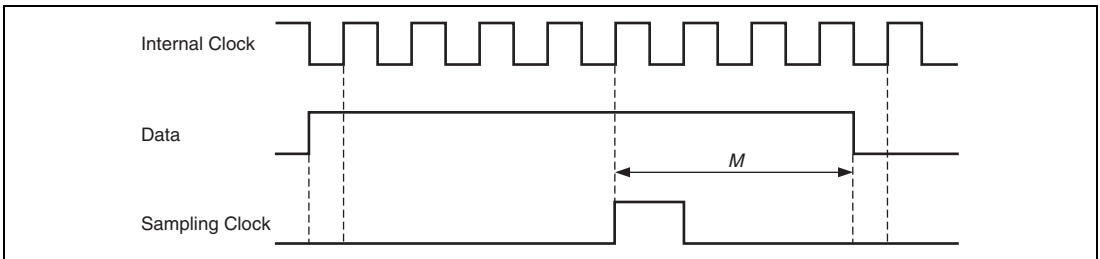
Figure 25.7 Receive Margin
