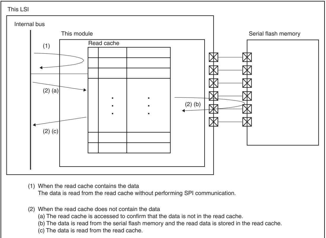
Figure 19.6 Burst Read Operation
