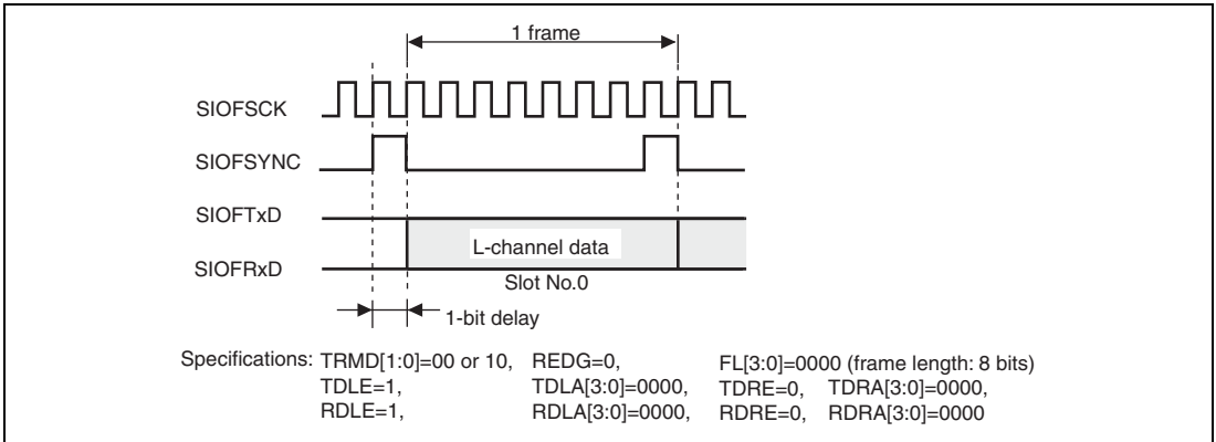
Figure 22.10 Transmit and Receive Timing (8-Bit Monaural Data (1))
