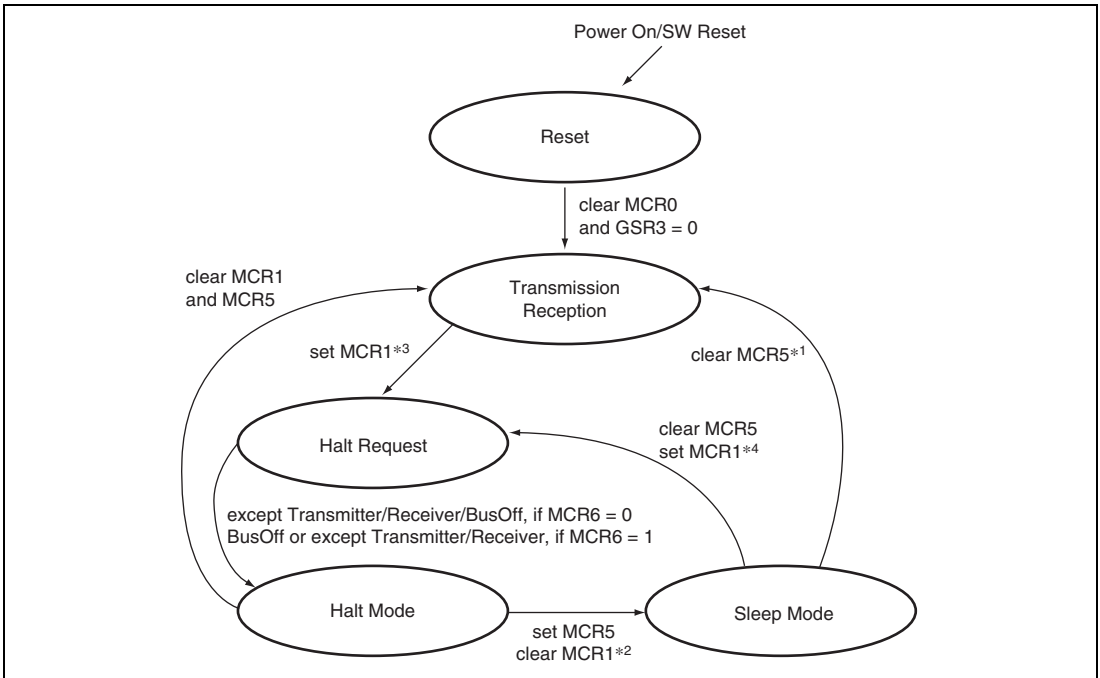
Figure 23.15 Halt Mode/Sleep Mode
