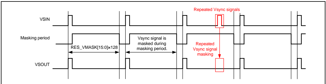
Figure 33.2 Timing for Masking Repeated Vsync Signals
