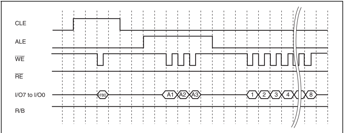
Figure 28.5 Programming Operation Timing for NAND-Type Flash Memory (1)
