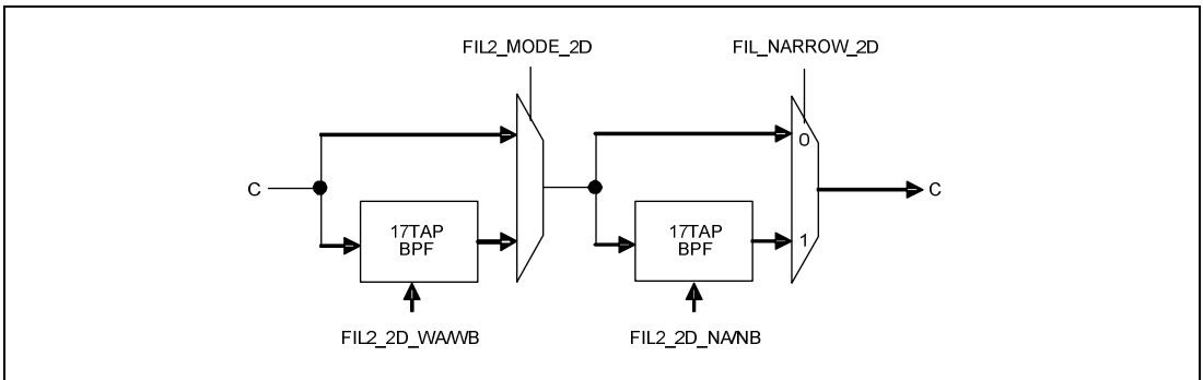
Figure 30.35 Configuration of Cascade Filter Block
