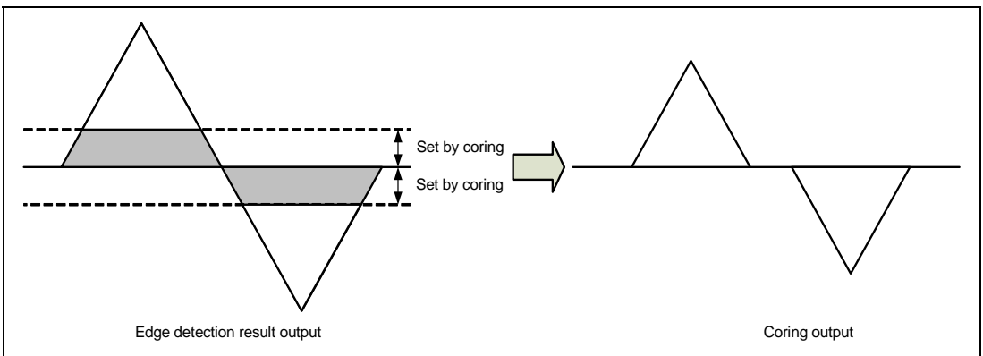
Figure 34.5 LTI Coring
