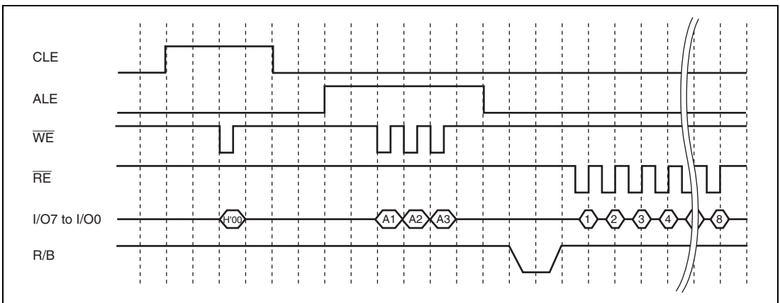
Figure 28.4 Read Operation Timing for NAND-Type Flash Memory
