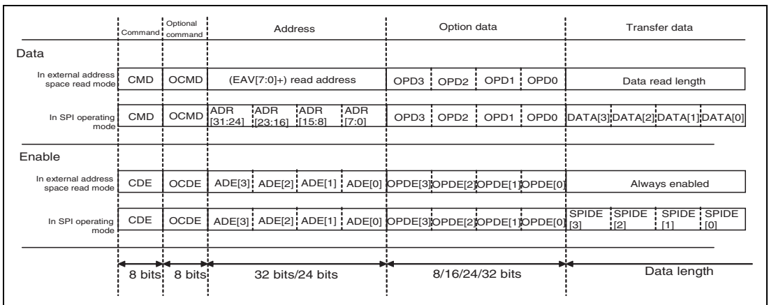
Figure 19.17 Data and Enable
