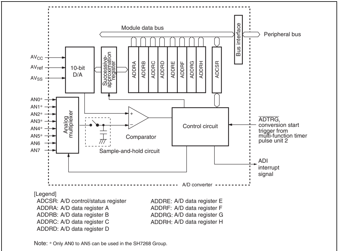
Figure 27.1 Block Diagram of A/D Converter
