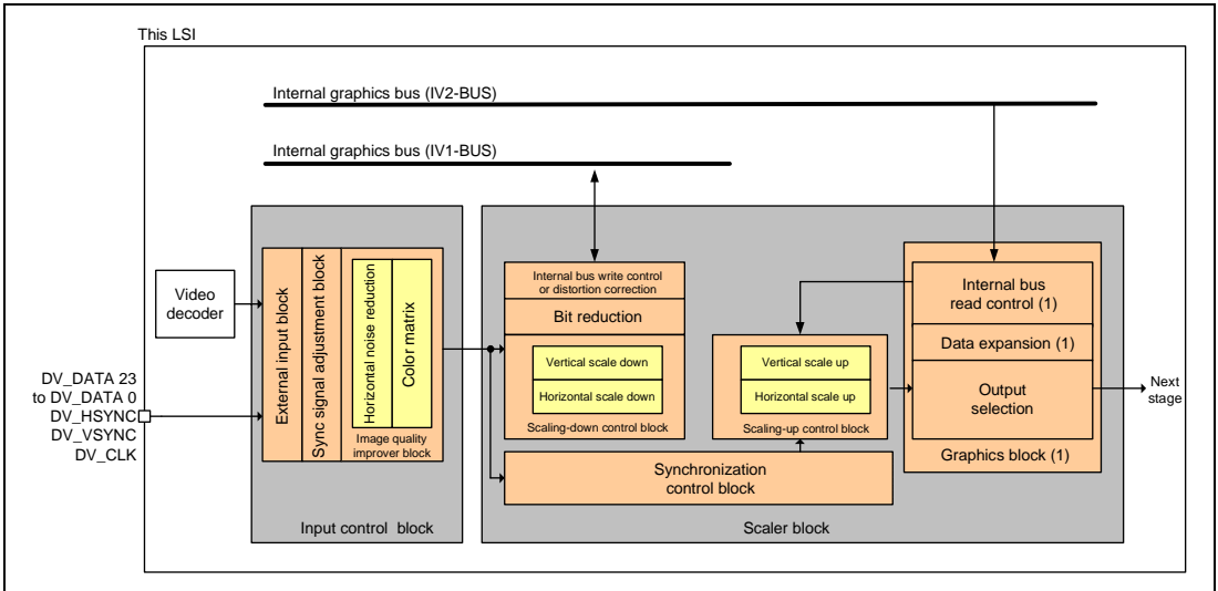
Figure 31.1 Video Display Controller 4 Former Stage Block Diagram
