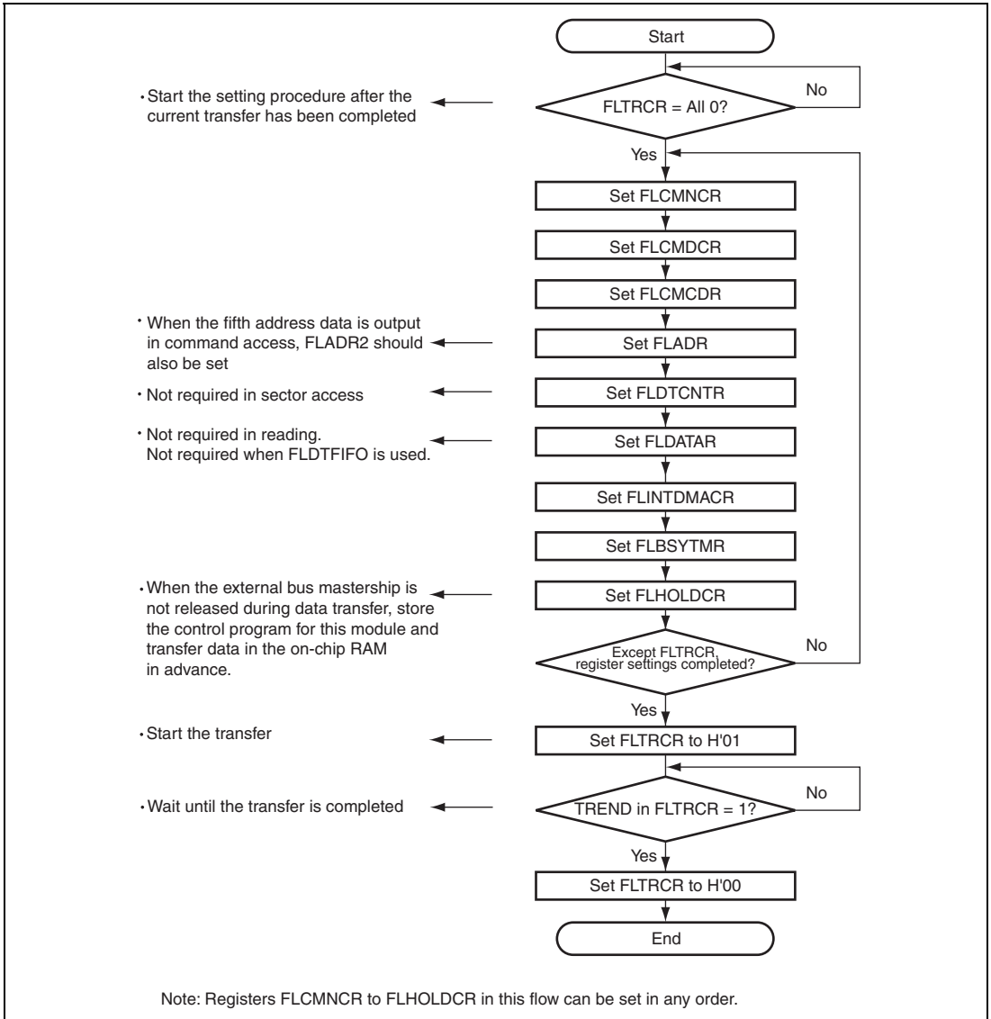
Figure 28.3 Register Setting Flow
