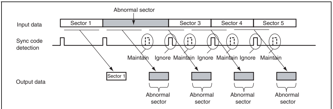
Figure 26.12 Operation in Interpolated Sync Mode
