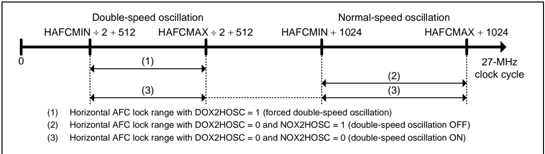
Figure 30.11 Horizontal AFC Lock Range (Horizontal)
