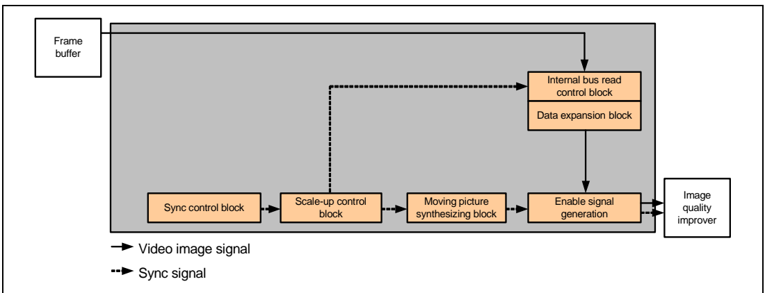
Figure 33.20 Signal Paths for Graphics Display
