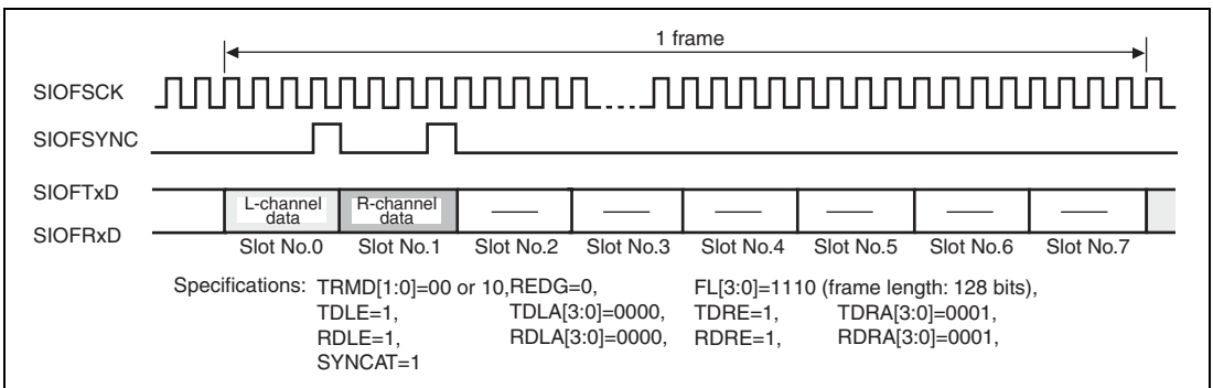
Figure 22.15 Transmit and Receive Timing (16-Bit Stereo Data)
