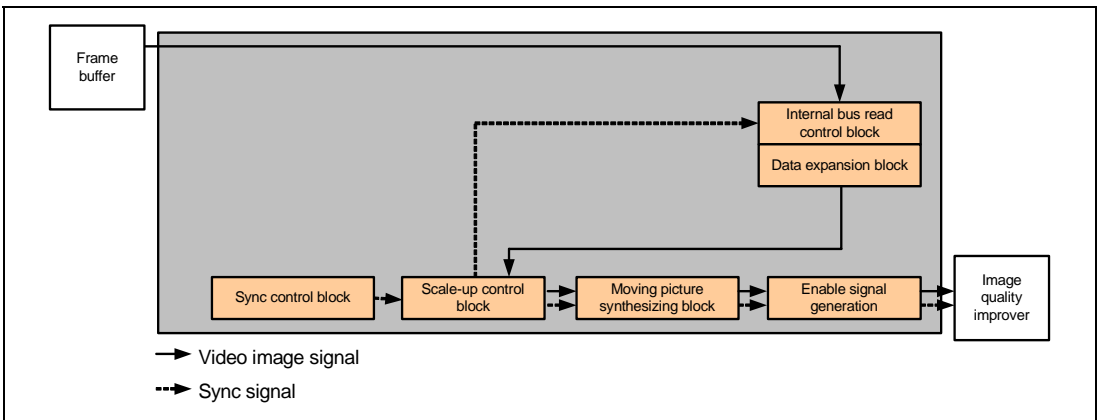
Figure 33.21 Signal Paths for Scaled-up Graphics Display
