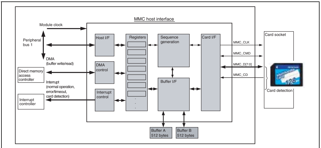
Figure 45.1 Block Diagram of MMC Host Interface
