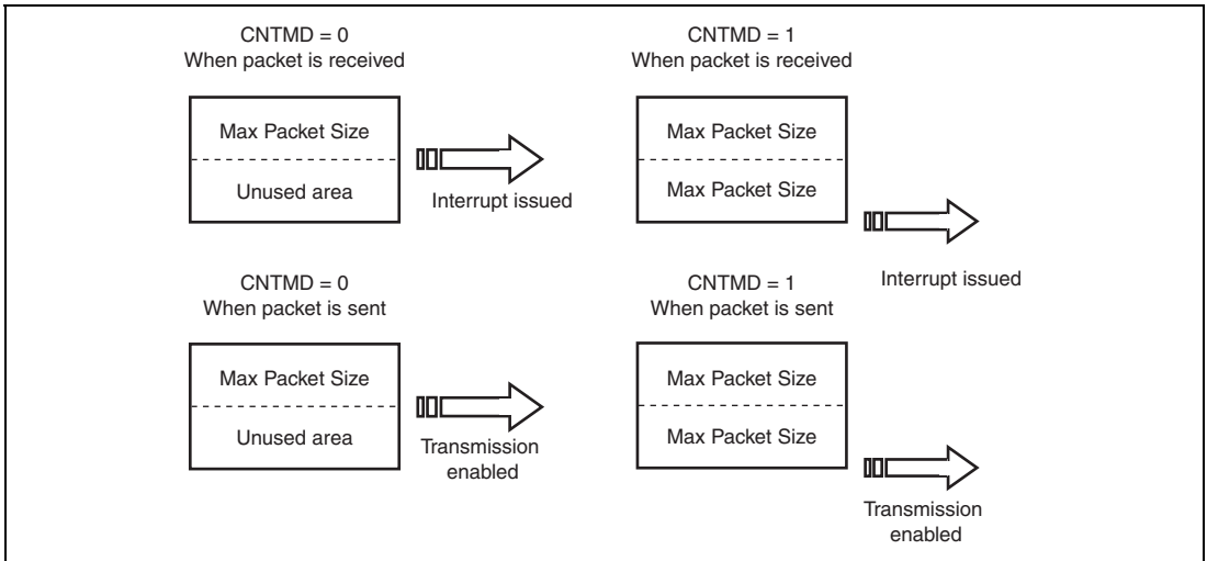
Figure 29.11 Example of Buffer Memory Operation
