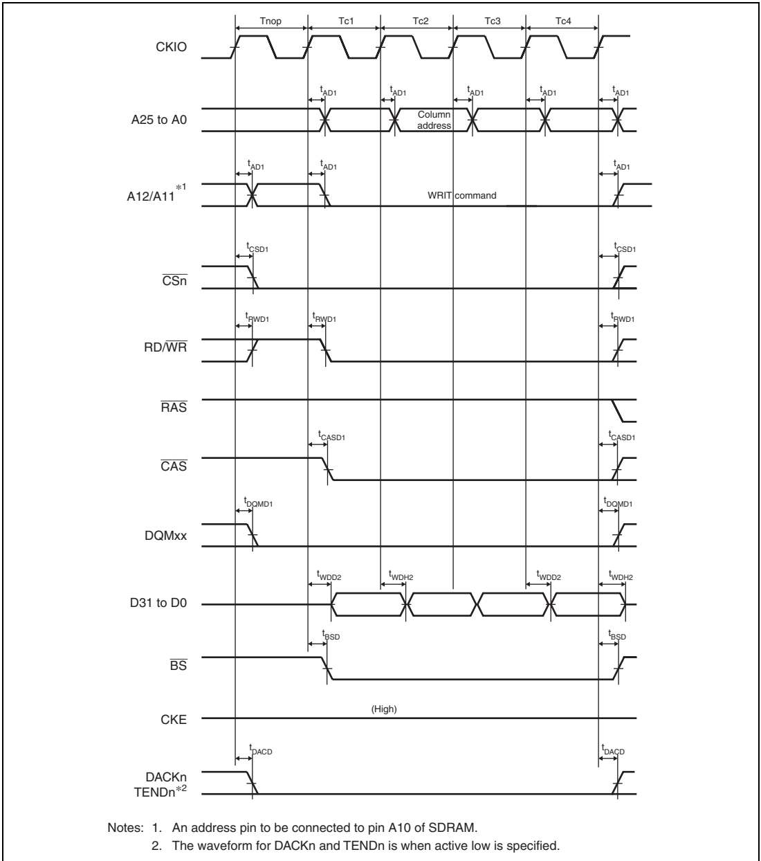
Figure 52.29 Synchronous DRAM Burst Write Bus Cycle (Four Write Cycles) (Bank Active Mode: WRITE Command, Same Row Address, WTRCD = 0 Cycle, TRWL = 0 Cycle)
