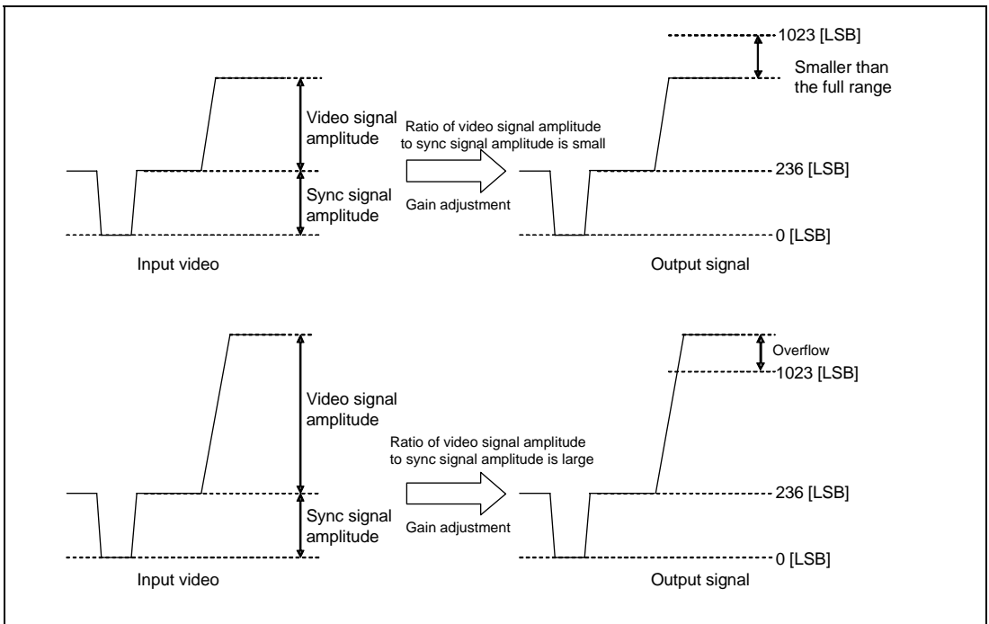
Figure 30.29 Cases in which Ratio of Video Signal Amplitude to Sync Signal Amplitude is Inappropriate
