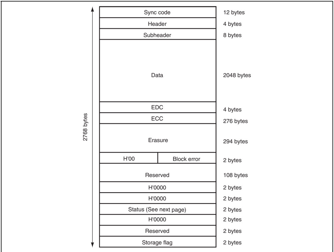
Figure 26.15 Output Data Stream Format
