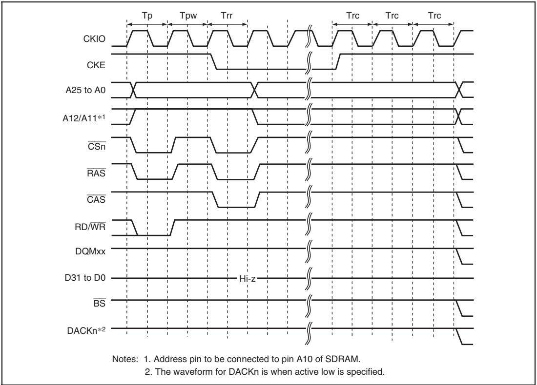
Figure 10.28 Self-Refresh Timing
