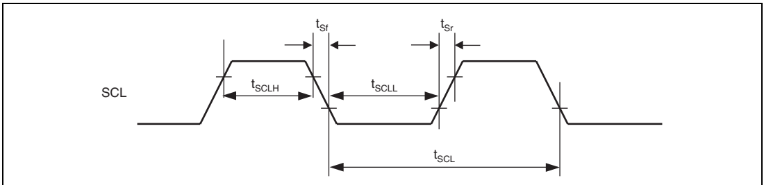
Figure 52.58(2) Clock Input/Output Timing
