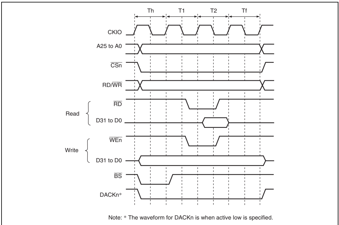
Figure 10.10 \overline{CSn} Assert Period Expansion
