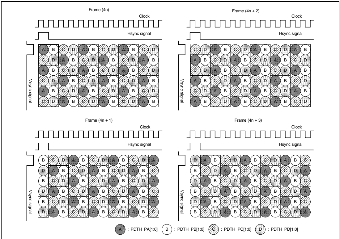
Figure 36.4 Operation Specification of 2 \times 2 Pattern Dither
