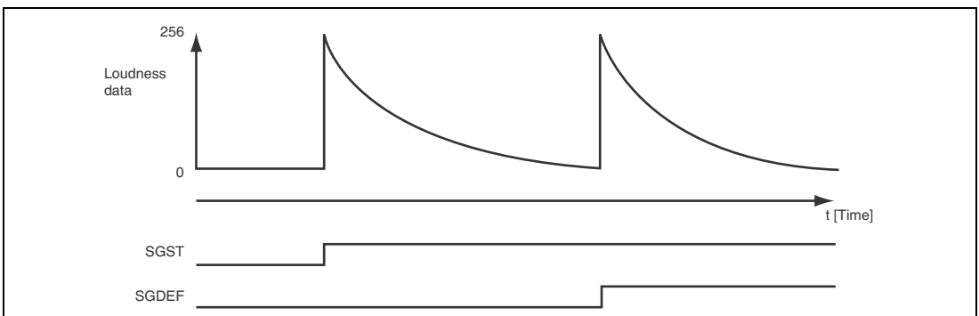
Figure 43.6 Attenuation End Flag Setting Timing
