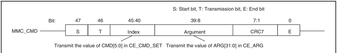
Figure 45.2 Command Format
