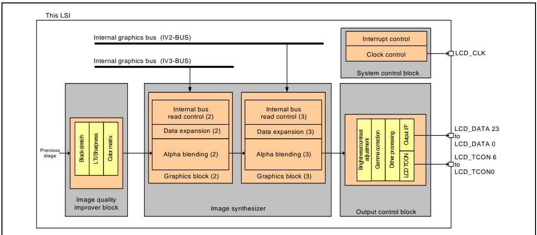
Figure 31.2 Video Display Controller 4 Latter Stage Block Diagram
