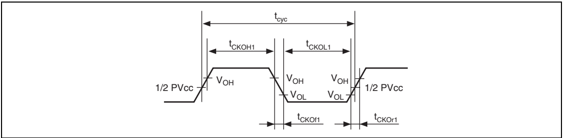
Figure 52.2 (1) CKIO Clock Output Timing 1
