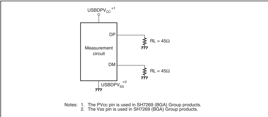
Figure 52.76 Measurement Circuit (High-Speed)
