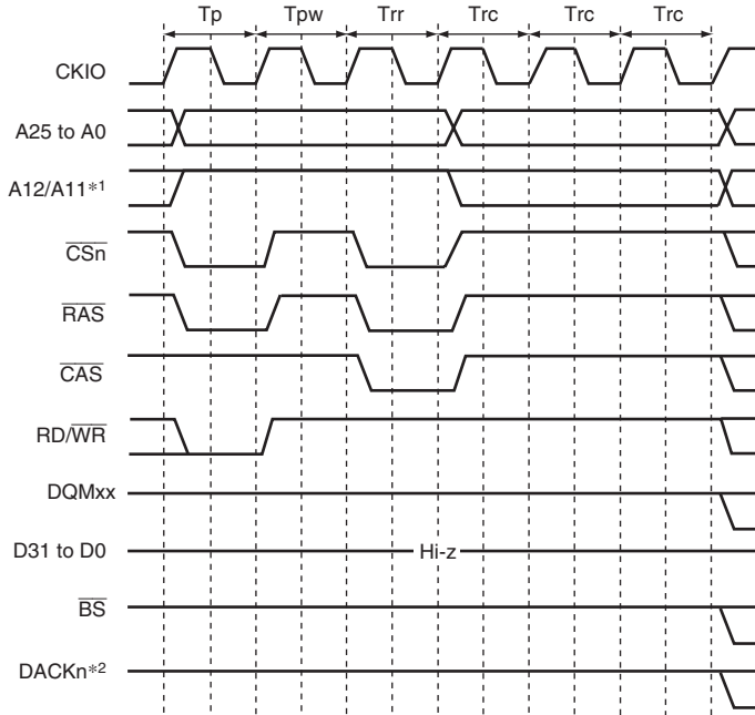
Figure 10.27 Auto-Refresh Timing
