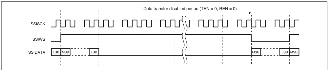
Figure 21.21 WS Continue Mode Disabled
