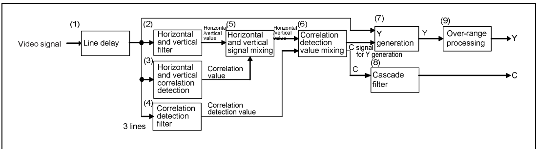
Figure 30.31 Block Diagram of Y/C Separator Circuit
