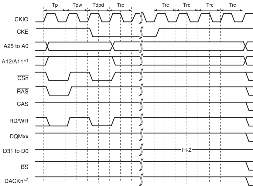
Figure 10.32 Deep Power-Down Mode Transition Timing
