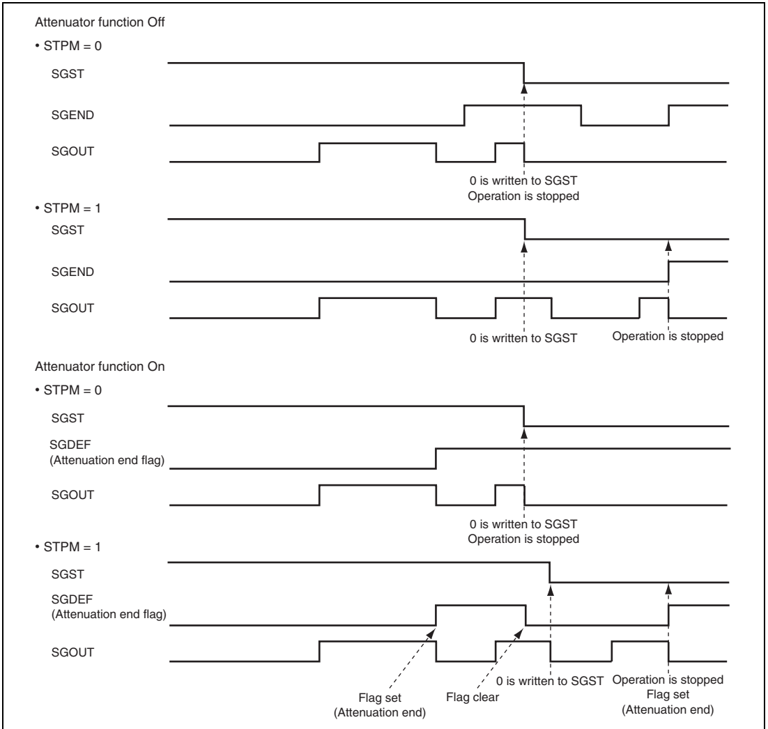
Figure 43.2 Examples of Stopping Operation
