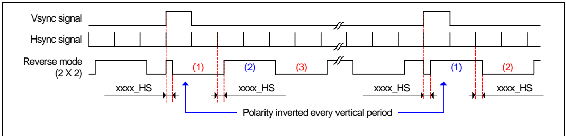
Figure 36.15 Horizontal Panel Driver Signal (in 2 × 2 Reverse Mode)
