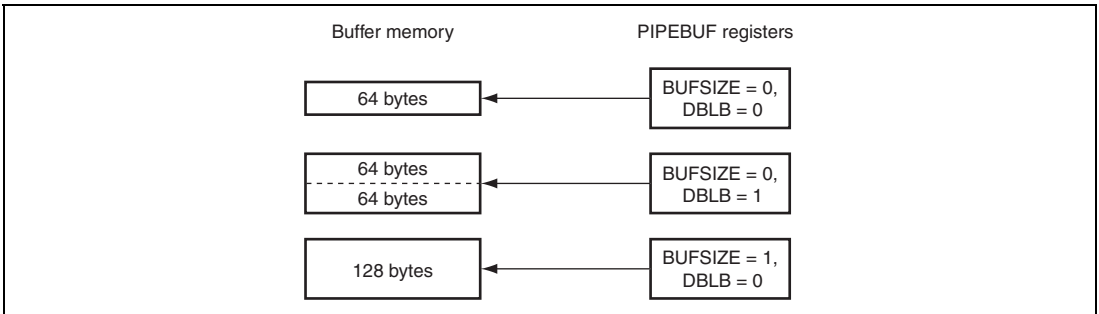
Figure 29.10 Example of Buffer Memory Settings
