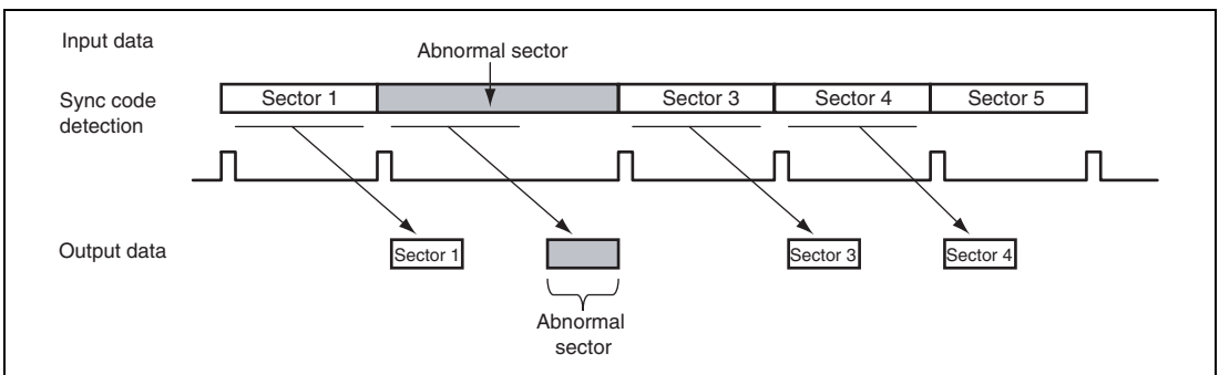
Figure 26.11 Operation in External Sync Mode
