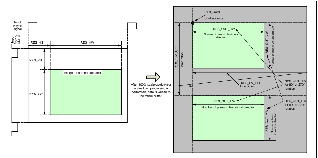
Figure 33.14 Data Arrangement in Frame Buffer
