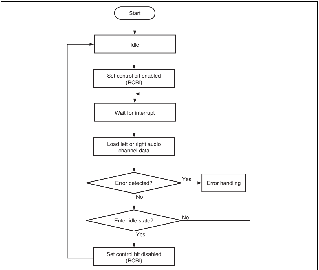
Figure 25.8 Receiver Data Transfer Flow Diagram - Interrupt Driven
