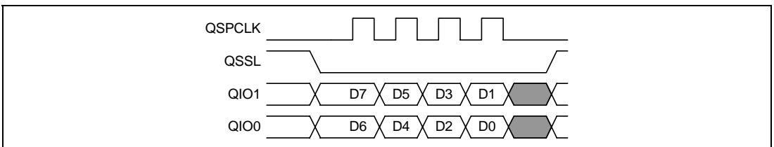
Figure 18.3 Transfer Format in Dual-SPI Format
