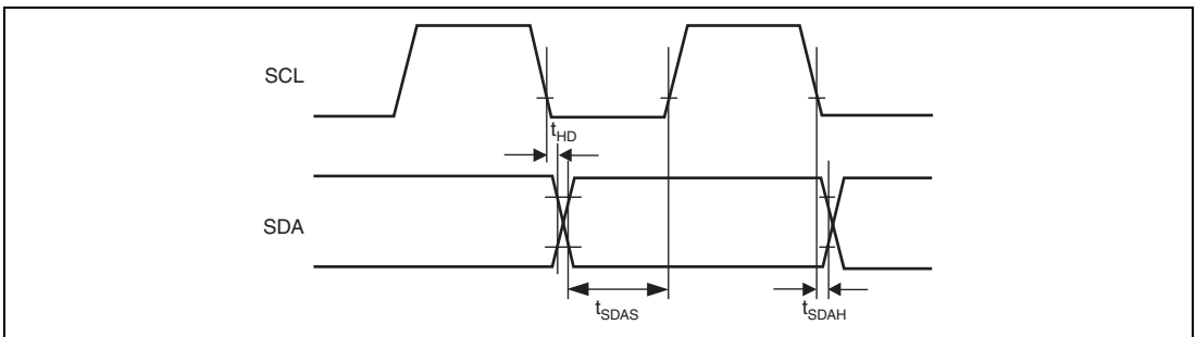
Figure 52.58(3) Transmission/Reception Timing
