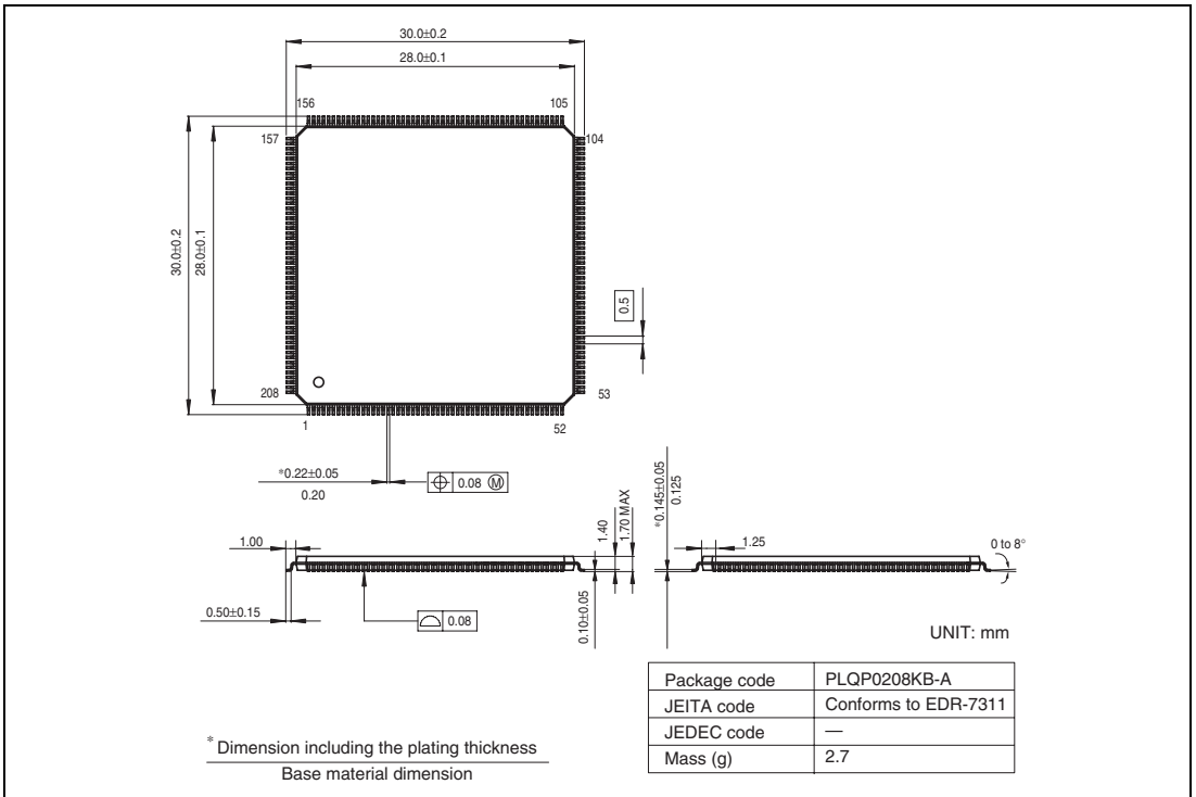
Figure A.1 SH7268
