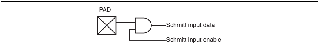
Figure 1.3 (2) Simplified Circuit Diagram (TTL AND Input Buffer)
