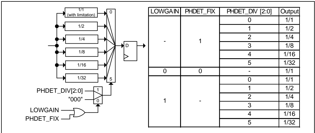
Figure 30.24 Phase Comparator Feedback Adjust
