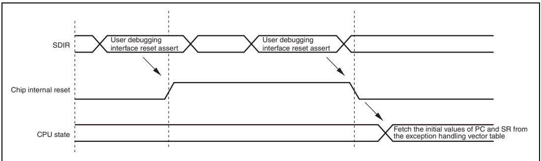
Figure 50.4 User debugging interface Reset
