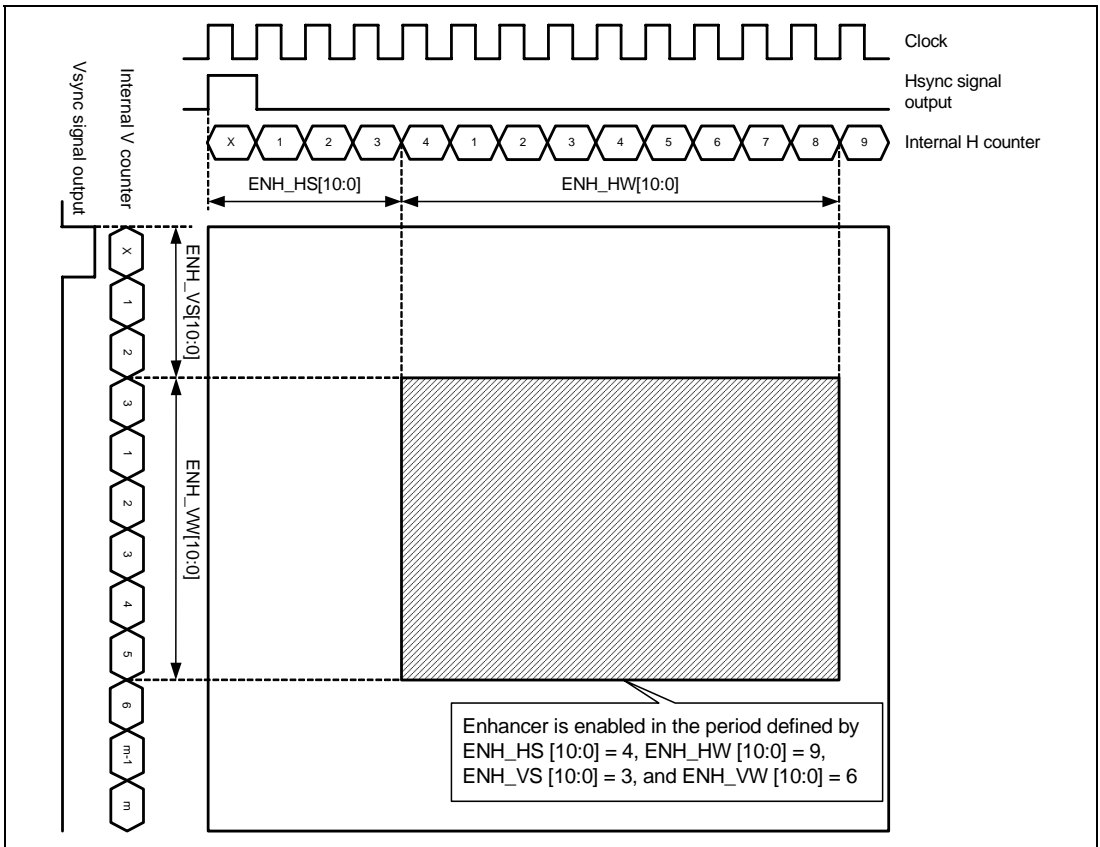
Figure 34.3 Period when Enhancer is Enabled
