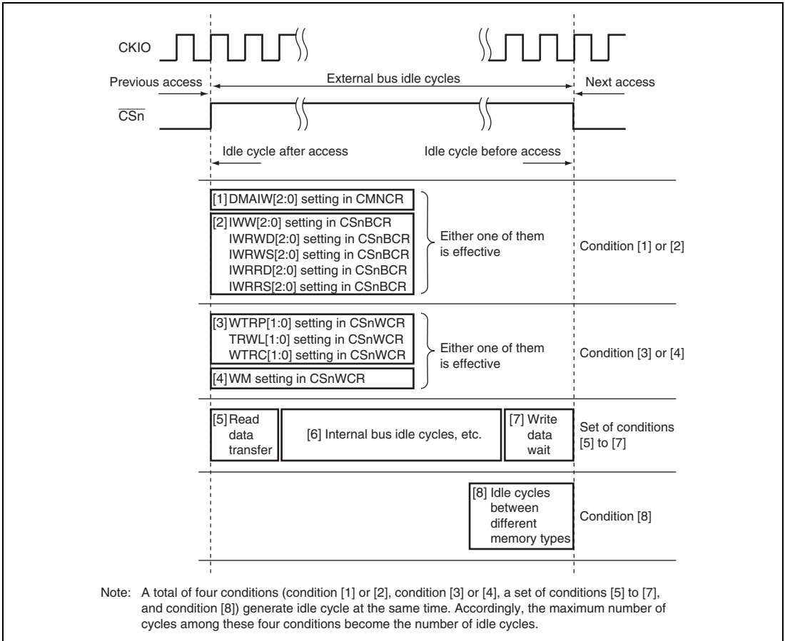
Figure 10.46 Idle Cycle Conditions
