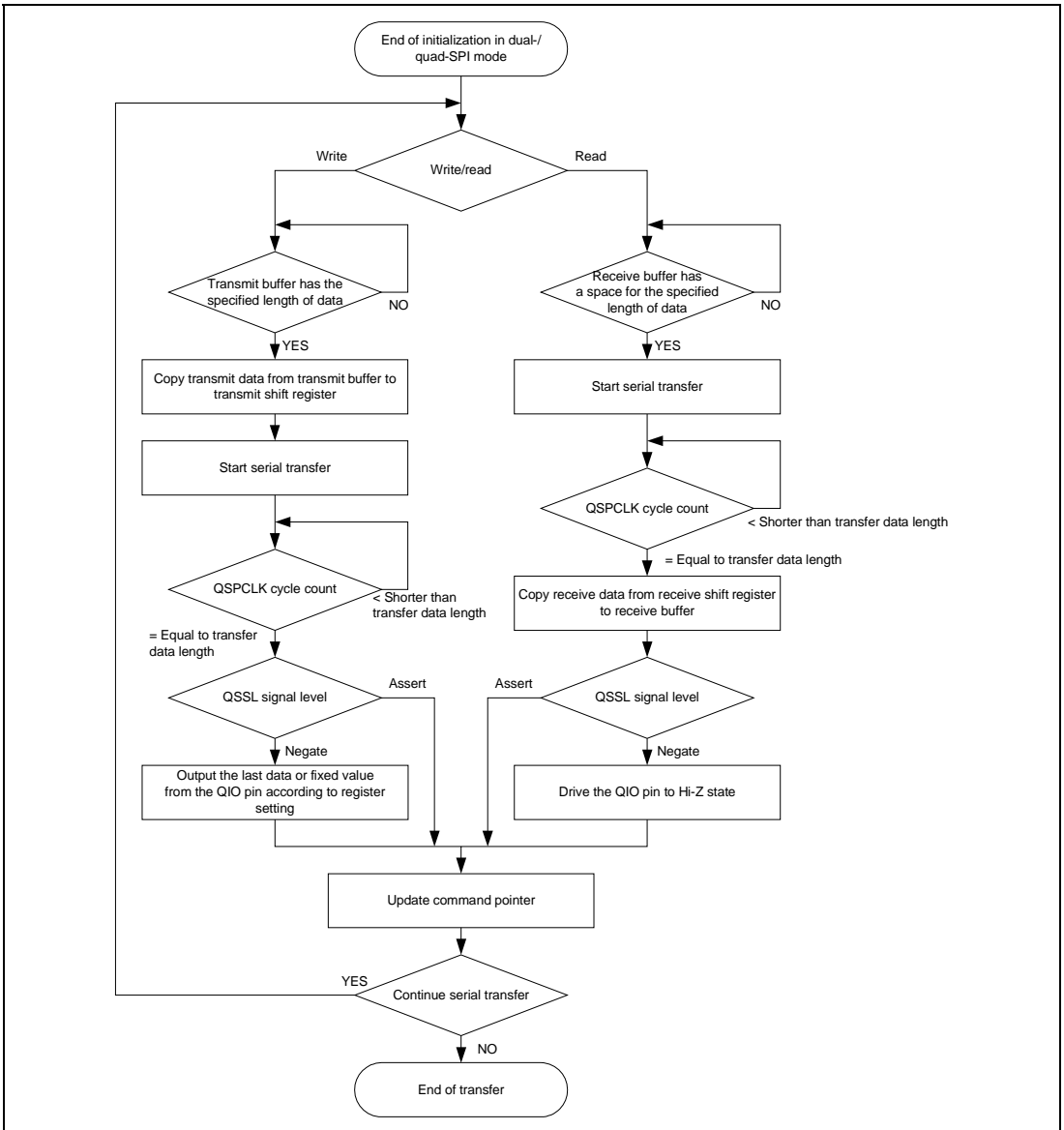
Figure 18.21 Transfer Operation Flowchart in Dual-/Quad-SPI Mode
