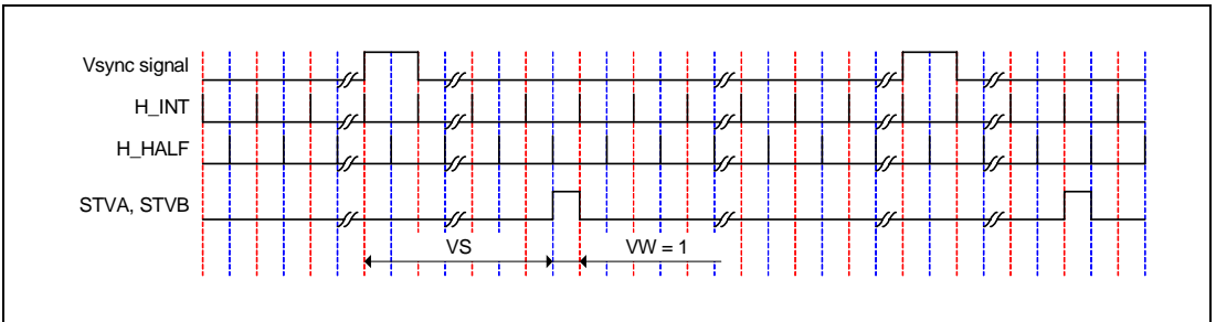
Figure 36.19 Vertical Panel Driver Signal (H_INT and H_HALF Reference Operation)
