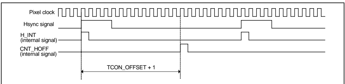
Figure 36.9 Generation of Offset Horizontal Reference (H_OFF) Signal
