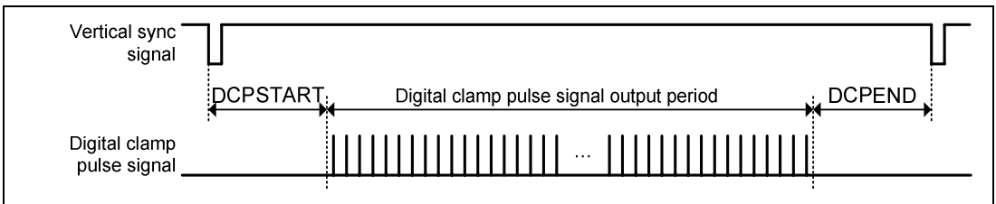
Figure 30.14 Digital Clamp Timing (Vertical)
