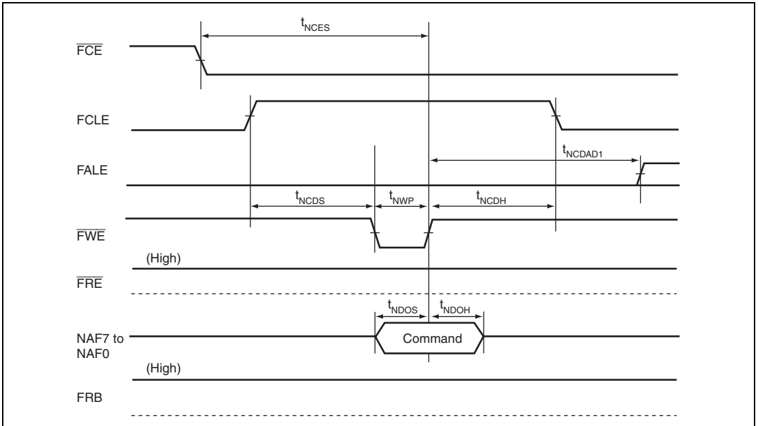
Figure 52.66 NAND Type Flash Memory Command Issuance Timing
