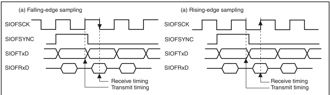
Figure 22.4 Transmit/Receive Timing
