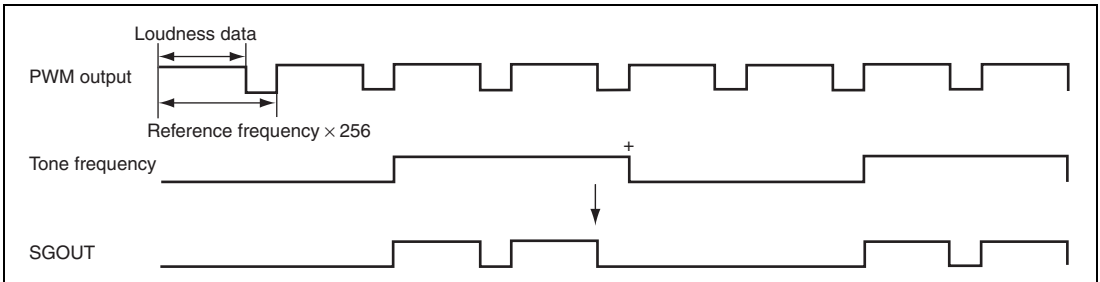
Figure 43.5 Output Waveforms
