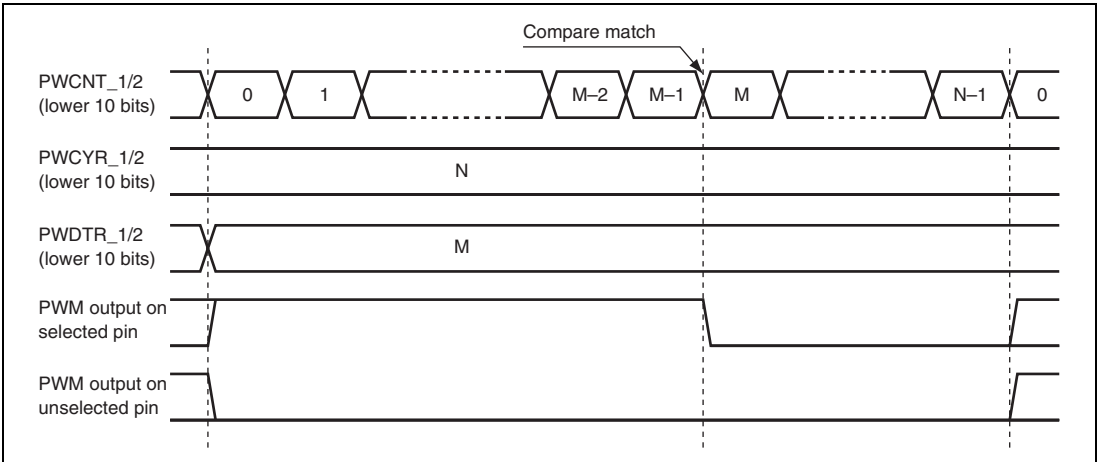
Figure 46.3 Duty Register Compare Match (OPS = 0 in PWPR_n)
