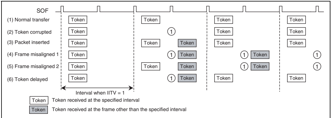
Figure 29.22 Example of an Interval Error Being Generated when IITV = 1
