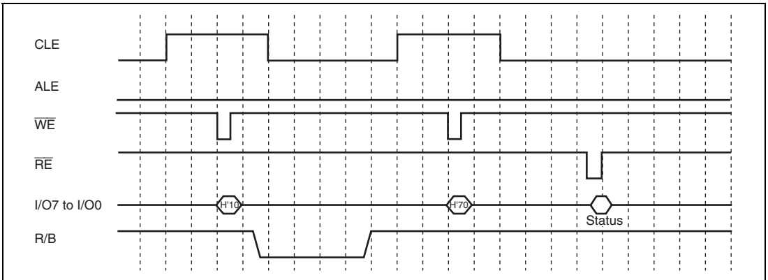
Figure 28.6 Programming Operation Timing for NAND-Type Flash Memory (2)
