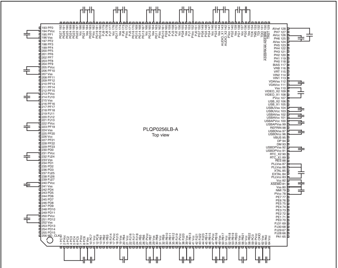
Figure 53.2 Example of Externally Allocated Capacitors in the SH7269 (QFP) Group
