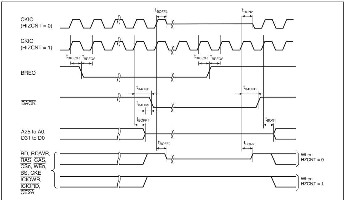
Figure 52.8 Bus Release Timing
