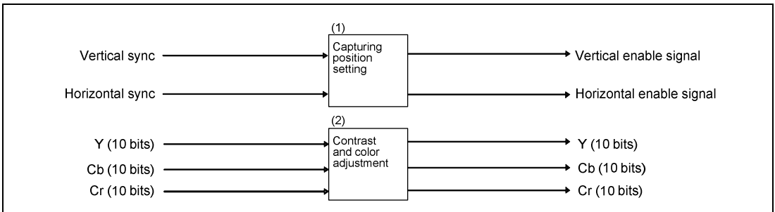
Figure 30.38 Block Diagram of Output Control Circuit
