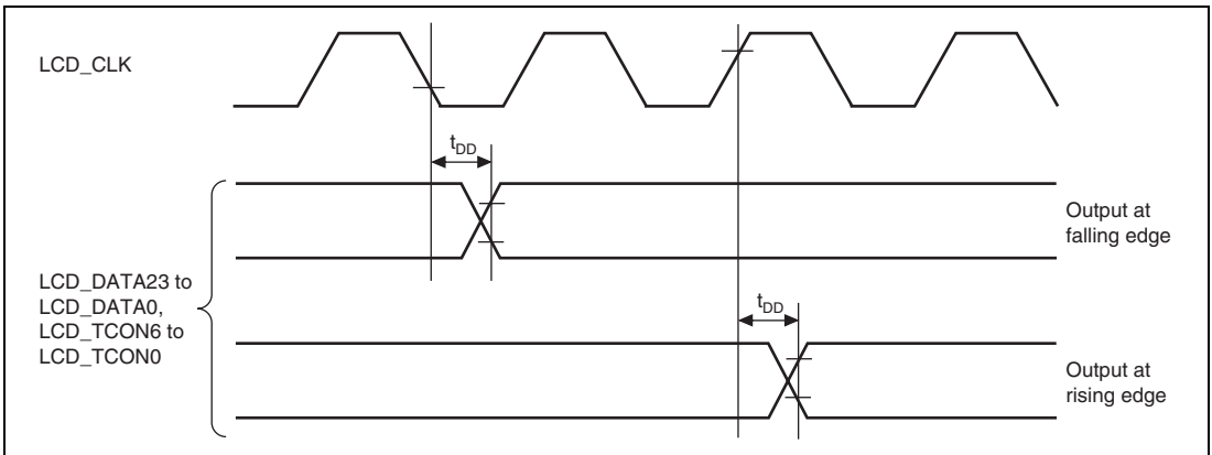
Figure 52.80 Display Output Timing
