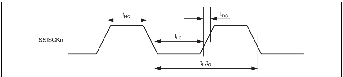
Figure 52.59 Clock Input/Output Timing
