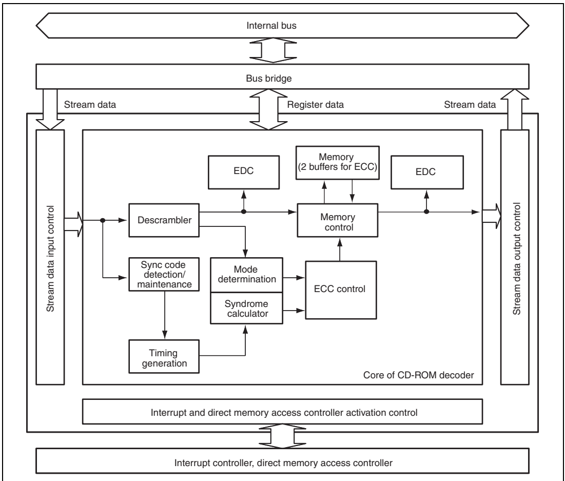
Figure 26.2 Block Diagram
