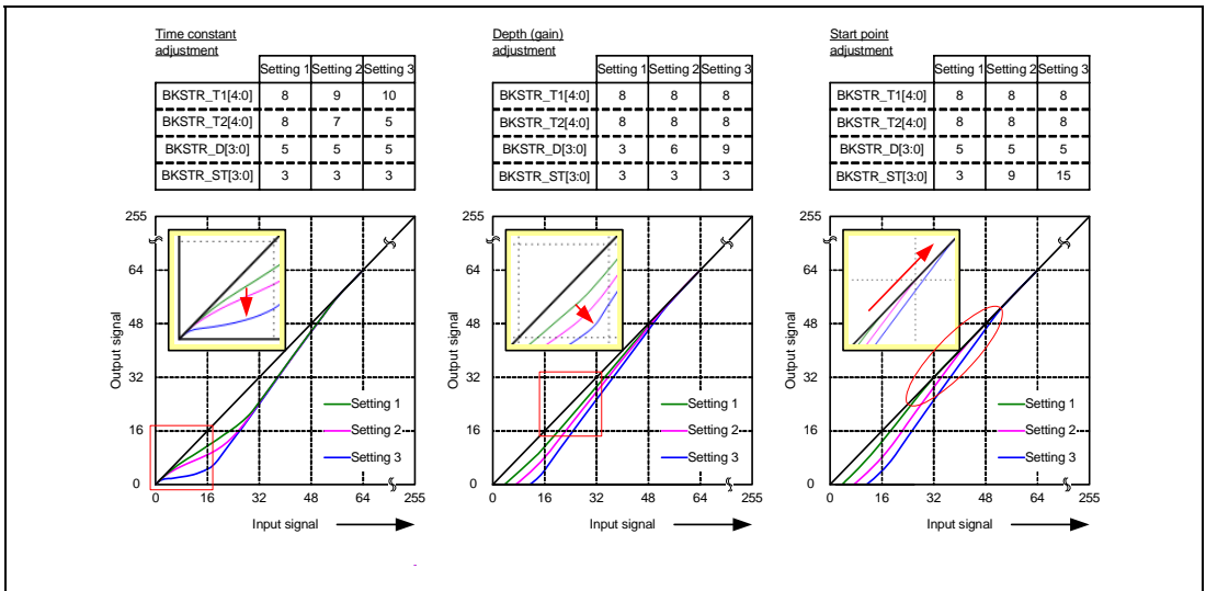
Figure 34.2 Black Stretch Correction (With Sample Settings)
